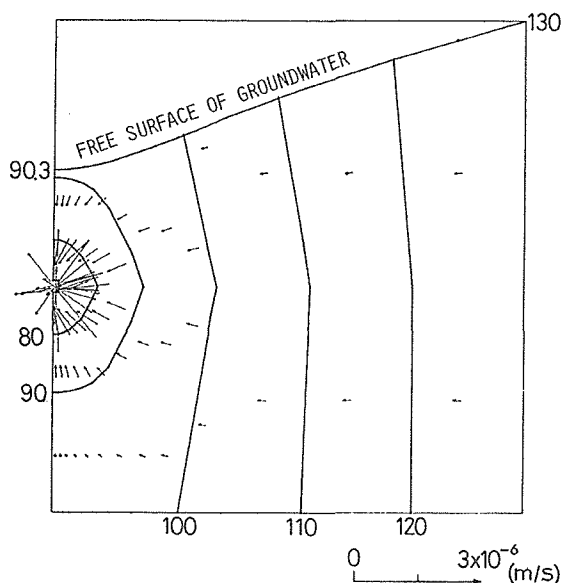
Fig. 11 State of groundwater flow in 360th day from the start of water drainage.
