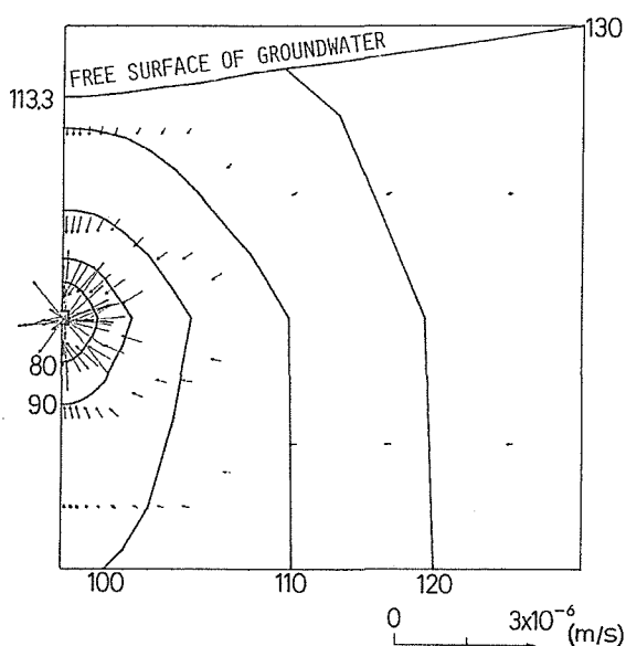
Fig. 10 State of groundwater flow in 20th day from the start of water drainage.
