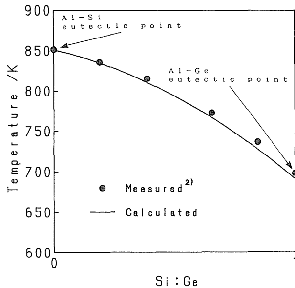
Fig. 3 Monovariant temperature curve from binary Al-Si eutectic point to binary Al-Ge eutectic point in the Al-Ge-Si ternary system.
