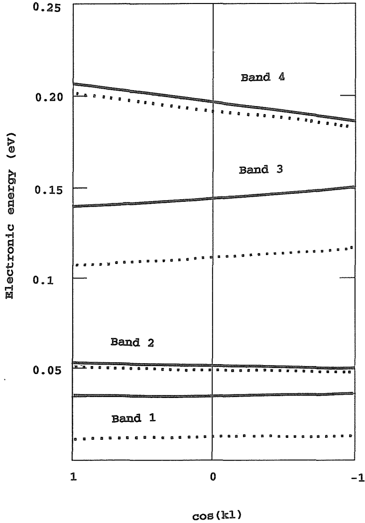
Fig. 7 Numerical results of the band structures in a AB-type superlattice structure. Dotted line is the results of simple Kronig - Penny type bands with a=50 \text{ \AA} , b=180 \text{ \AA} , and Va=0.25 \text{ eV} .
