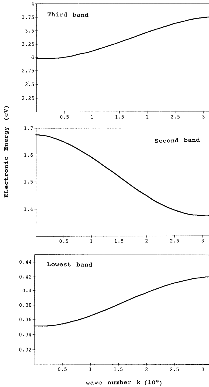
Fig. 3(a) An example of Kronig - Penny Band. V=4.5 eV, a=2 Å, and b=8 Å.
