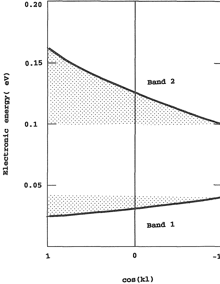
Fig. 4(b) Plot of energy versus \cos(kl) of the superlattice. Va=0.25 eV, a=20 Å, and b=100 Å.
