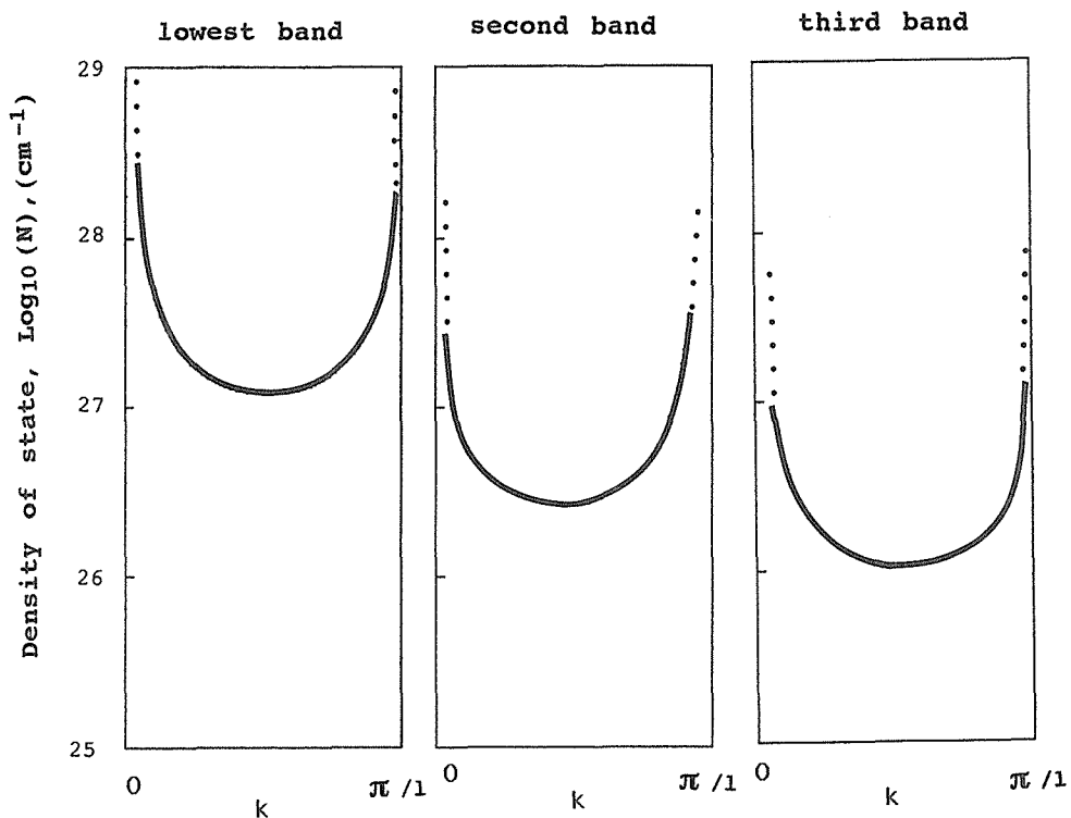
Fig. 3(b) The density of state for the bands in Fig. 3(a).
