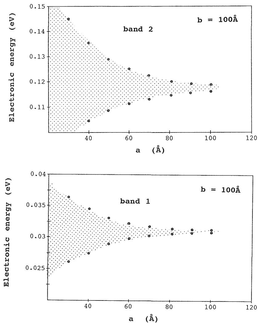
Fig. 5 The variation of the width of conduction band as a function of the width of potential barrier a .
