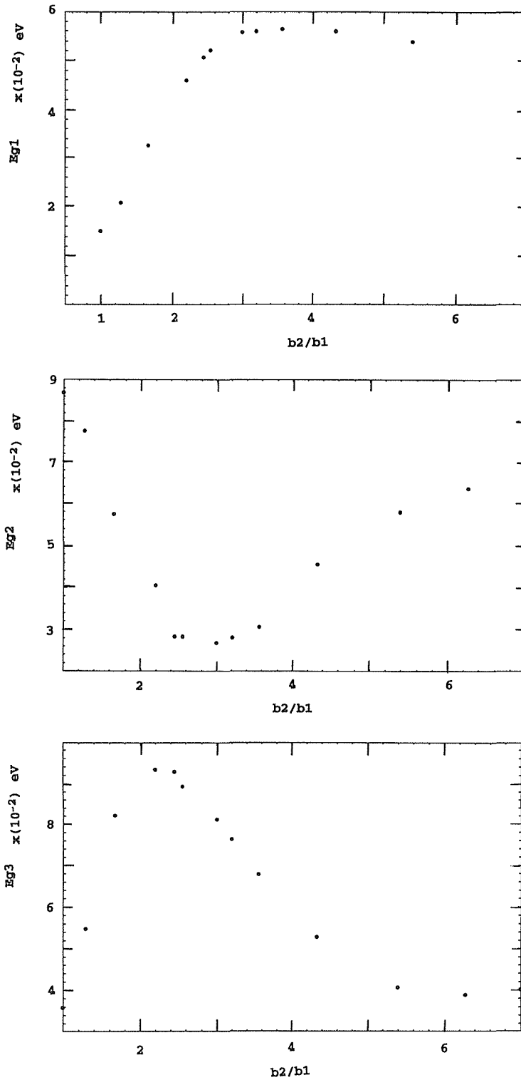
Fig. 8(a), (b), and (c) Variations of energy gaps as a function of the ratio w = b_2/b_1 .
