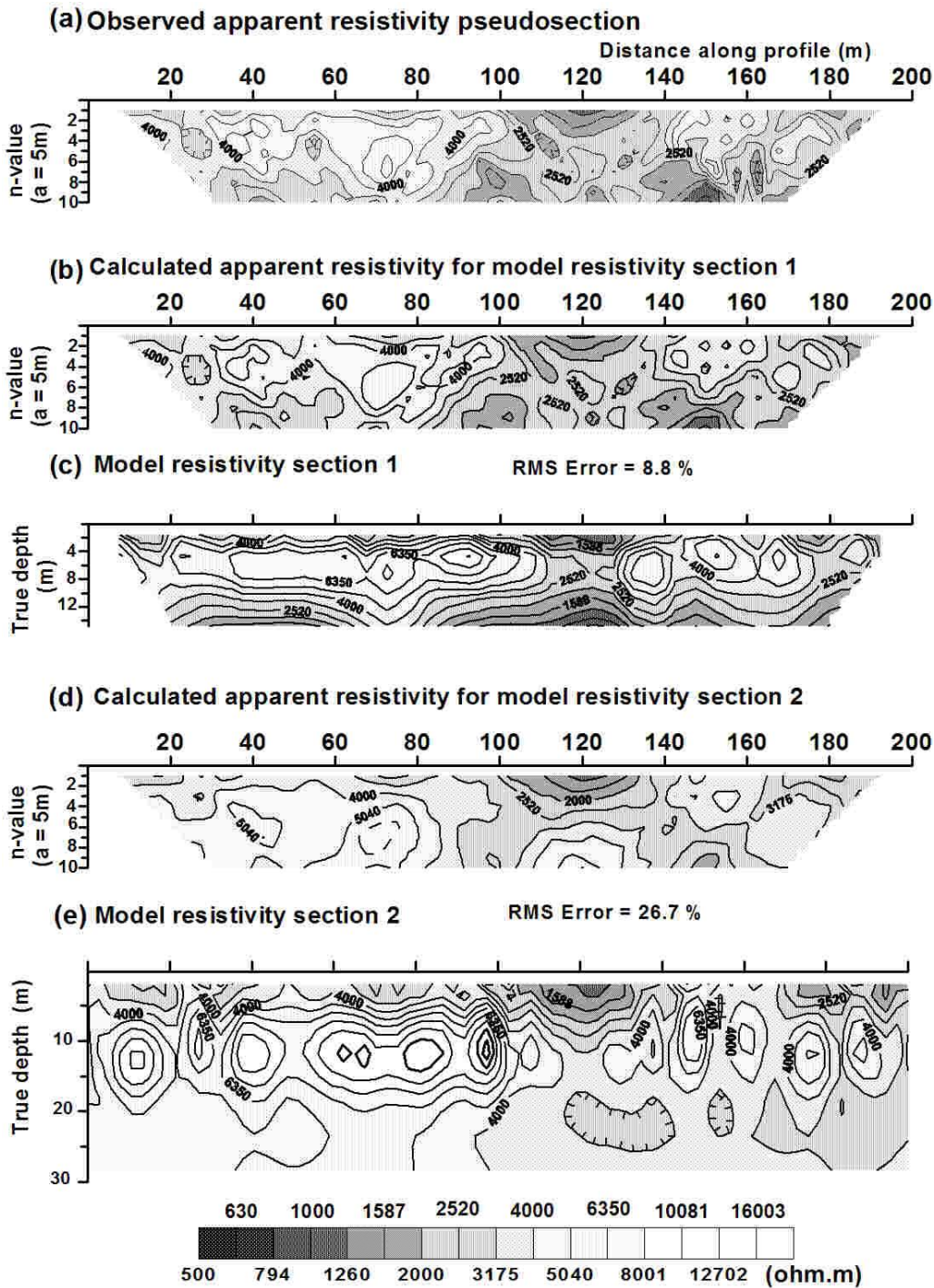
Fig. 6. Results of electrical imaging by dipole-dipole array along profile IP1 from the Powerhouse area (see Figs. 2. and 5 for profile location). (a): Measured data ; (b)- (c): Results of 2D-inversion following the scheme of Loke and Barker (1996); and (d)-(e): Results of 2D-inversion after Dietrich (1999). Though the models show similar shapes, the depth distribution of objects of contrasting resistivity differs significantly. Model section (c) is the best mathematical solution as it has low \epsilon_{RMS} . The model section (e) is a second choice on the basis of \epsilon_{RMS} but seems to be a closer match to the observed and expected depth of distribution of the buried void spaces characterized by elevated resistivities.
