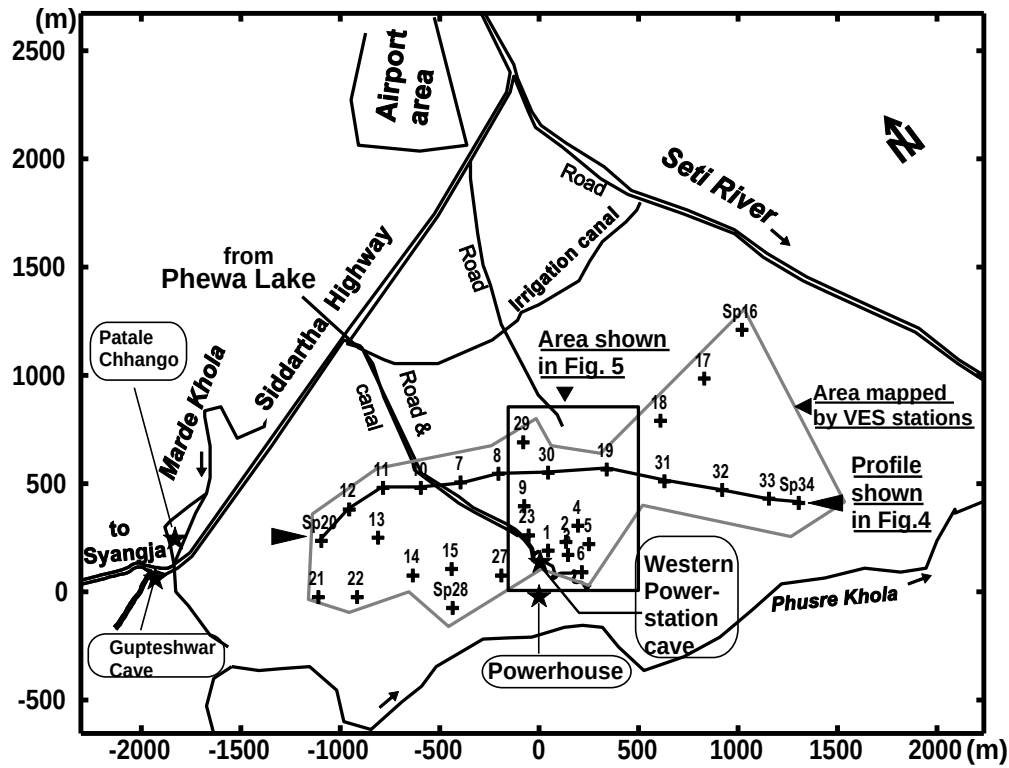
Fig. 2. The Powerhouse- Chhorepatan area. Locations of major caves (stars: Patale Chhango or Devi's Fall, Gupteshwar cave, western PowerStation cave). The irregular polygon shows the area studied by electrical sounding (ES). The stations are identified by numbers (for clarity, only a few of them are preceded by "Sp" meaning sounding point).
