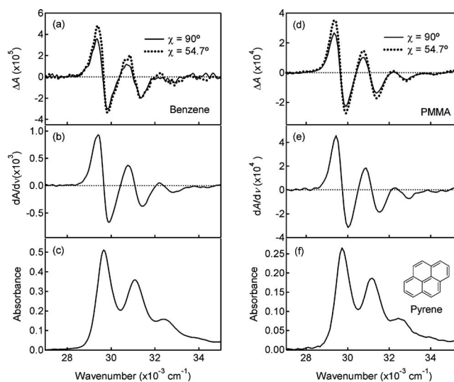
FIG. 7. Absorption and EA spectra of pyrene in benzene (left) and in PMMA (right). [(a) and (d)] EA spectra observed with \chi=90^\circ (solid line) and \chi=54.7^\circ (dotted line), [(b) and (e)] the first derivative of the absorption spectrum, and [(c) and (f)] absorption spectrum observed with \chi=90^\circ . The applied field strength was 0.10 \text{ MV cm}^{-1} in benzene and 1.0 \text{ MV cm}^{-1} in PMMA. Molecular structure of pyrene is shown in the figure.
