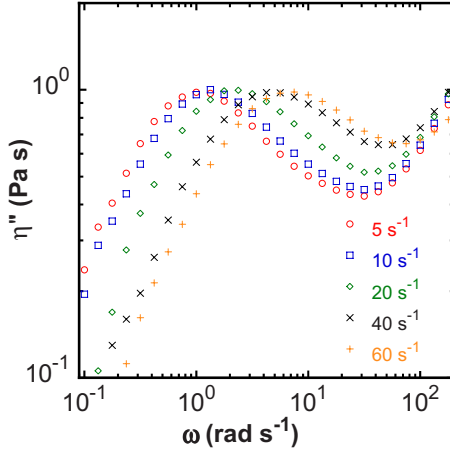
FIG. 6. (Color online) Frequency dispersions of out-of-phase viscosity for the LCP/DMS blend after applying preshears of 5, 10, 20, 40, and 60 s -1 , respectively.
