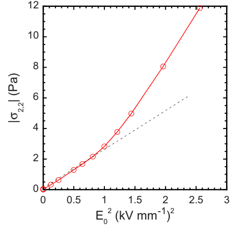
FIG. 2. (Color online) Dependence of |\sigma_{2,2}(\omega)| on the squared amplitude of ac electric field E_0^2 , at \dot{\gamma} = 20 \text{ s}^{-1} and \omega = 1.38 \text{ rad s}^{-1} .
