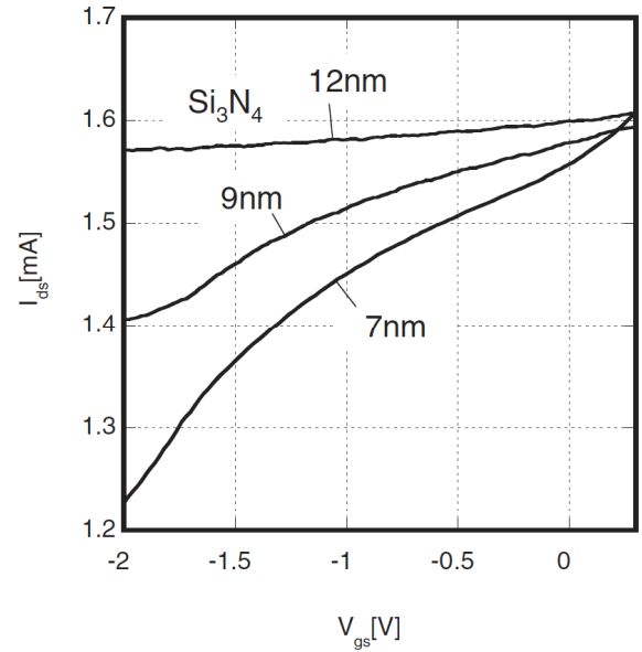
Fig. 7 I_{ds} - V_{gs} characteristics of open-gate FETs having \text{Si}_3\text{N}_4 films 7, 9, and 12 nm thick.
