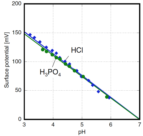
Fig.8 Relation between surface potential and pH values of electrolytes for InP-based open-gate FETs having \text{Si}_3\text{N}_4 films 7 nm thick.
