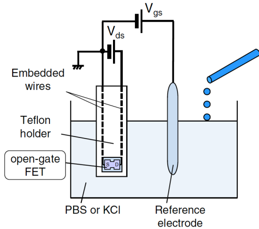
Fig. 2 Experimental setup for sensing measurements.
