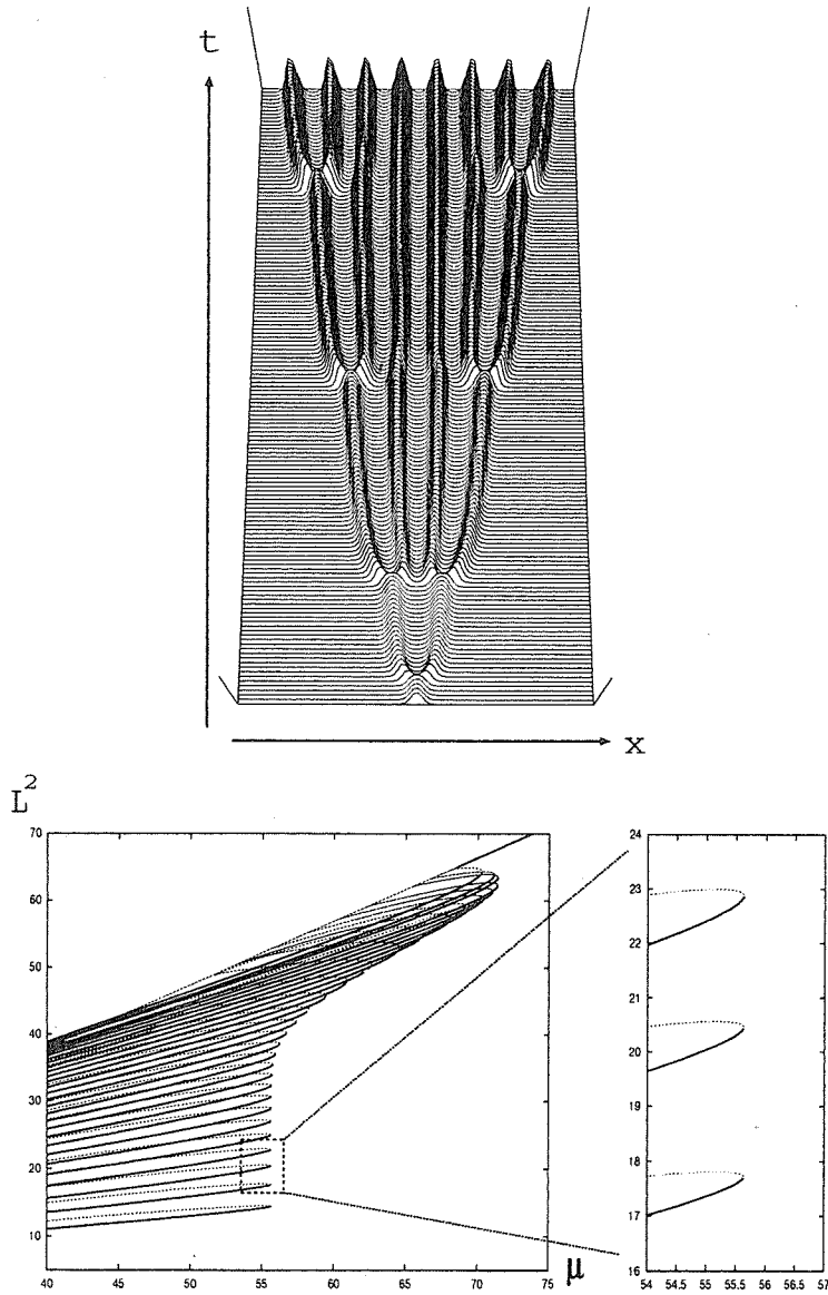
FIGURE 5. Self-replication dynamics for the Gierer-Meinhardt model. The upper picture shows the time-evolution of the replication process starting from a localized initial data. The global bifurcation diagram (below) with respect to the decay rate \mu shows the locations of saddle-node points for steady states of multi-hump type. The number of humps is increased from the bottom up. When the distance between humps is well-separated (i.e., lower branches), their locations coincide well; however, they don't coincide for higher modes due to the finite-size effect.
