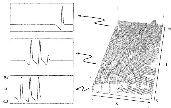
FIGURE 3. Self-destruction of triple-traveling-pulse oscillatory tail.
