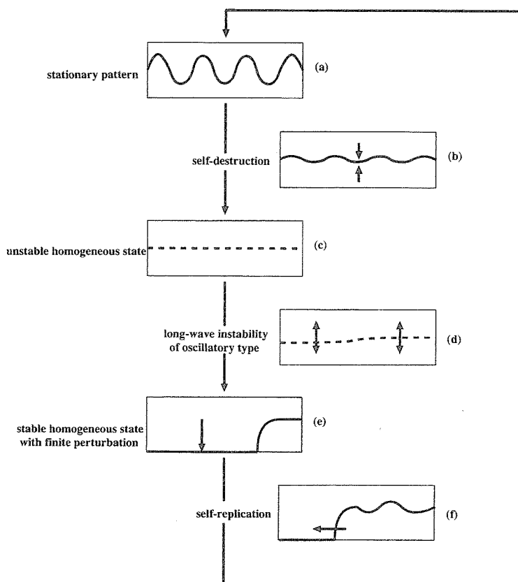
FIGURE 7. A generalized heteroclinic cycle for the Gray-Scott model. It consists of a spatially periodic pattern, an unstable constant solution P , and a stable constant state (u, v) = (1, 0) with localized perturbation. In a loose sense the orbit itinerates these patterns when the system size is large enough. More precisely a self-replication wave starts from a localized perturbation and forms a periodic pattern; however, it destructs to the homogeneous state P . The constant state has an oscillatory instability of long-wave type, the destination of this instability is the background state (1, 0) , but it converges non-uniformly due to the oscillatory nature; therefore there always exists a localized bump as in (e) other than the (1, 0) -state, which is the beginning of another cycle.
