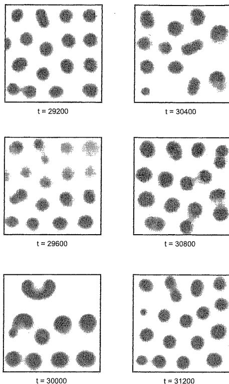
FIGURE 1. Two-dimensional spatio-temporal chaos for the Gray-Scott model. Each spot can replicate by itself. After the domain is filled by the spots, there occurs a competition searching for fresh substrate among them. The four spots in the top right start to disappear around t = 29600 and vanish completely at t = 30000 . The surrounding spots invade into the empty region and start to replicate there until the domain is filled by four islands again at t = 31200 . Self-replication and self-destruction successively occur in a chaotic manner.
