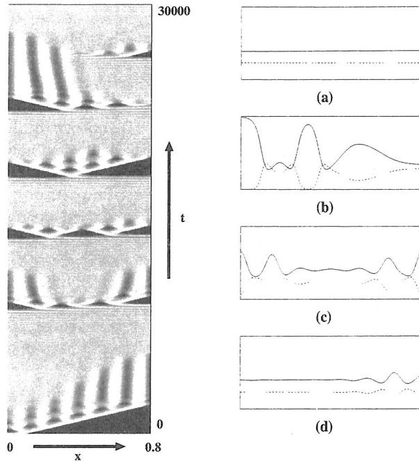
FIGURE 6. One-dimensional spatio-temporal chaos for the Gray-Scott model (gray-scale left) and typical profiles of u (solid line) and v (dotted line). It shows one cycle from an almost uniform state (a) to more or less the same state (d) via replication (b) and destruction (c).
