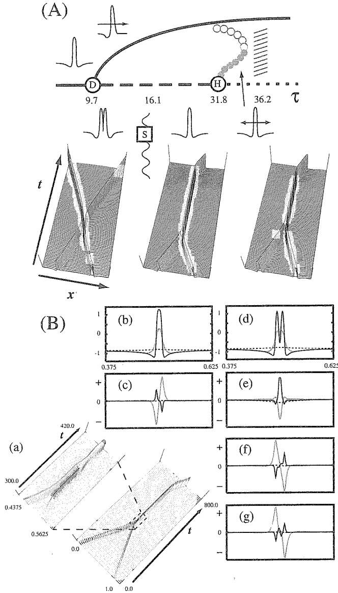
FIGURE 9. (A) Phase-diagram of scattering for the gas-discharge model. The three evolutions show 2 into 2 (reflection), 2 into 1 (coalescence) and 2 into 1 (coalescence with oscillation) (left: \tau = 15.0 , center: \tau = 20.0 , right: \tau = 35.0 ) respectively. (B) Two scatters and their heteroclinic connection: (a) When \tau is slightly larger than \tau^s , the orbit deforms along the heteroclinic connection from twin-horn scatter to single-horn one. (b), (c) Single-horn scatter and its unstable eigen-profiles. (d), (e)-(g) Twin-horn scatter and its three unstable eigen-profiles. The solid (gray, dotted) line shows the u -component ( v -component, w -component) respectively.
