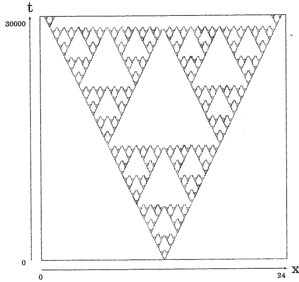
FIGURE 2. Spatio-temporal self-similar pattern for the Gray-Scott model (1) in which the v -component is shown in gray-scale. Self-replication and annihilation are balanced so that a Sierpinski-like self-similar pattern is produced. This was first found by Hayase-Ohta [10] for the reaction-diffusion system with the nonlinearity of Bonhoeffer-van der Pol type.
