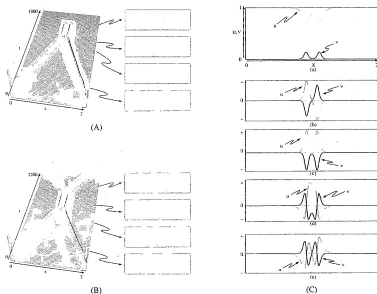
FIGURE 8. Scatter for reflection-annihilation transition and the associated eigenfunctions. As k is increased, the output is changed from annihilation (A) to reflection (B). Since both cases are very close to the transition point k_c , the profiles right after collision resemble the unstable steady state of twin-horn type depicted at the top of (C), called the twin-horn scatter. The linearized spectrum around it has three unstable eigenvalues besides the zero eigenvalue coming from translation invariance; i.e., their real parts are positive and the associated eigenfunctions are given as (a)-(c). The second symmetric case (b) plays a key role for head-on collisions.
