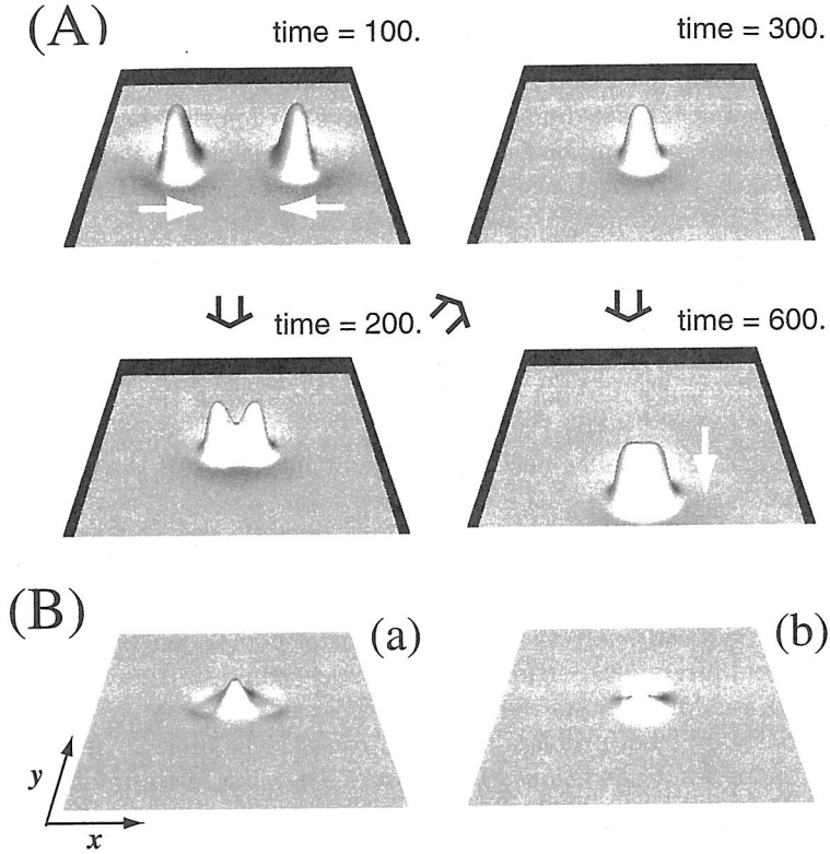
FIGURE 10. (A) Scattering of traveling spots (only u -component is shown). (B) Profiles of the unstable eigenfunction \phi_1 for the largest eigenvalue: (a) peanut scattor, (b) single-horn scattor, respectively.
