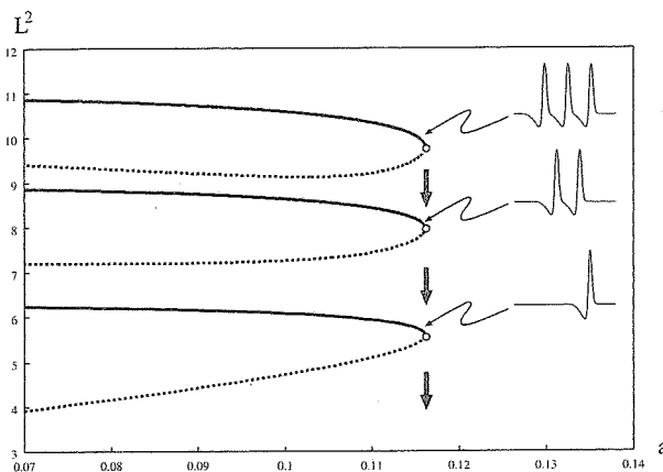
FIGURE 4. Global bifurcation diagram for the self-destruction process of a triple-traveling-pulse with an oscillatory tail. The horizontal axis is the threshold parameter a and the vertical axis is the L^2 -norm of the solution. The locations of single, double and triple pulses coincide with each other with high accuracy. Successive destruction occurs in the right part of this location.
