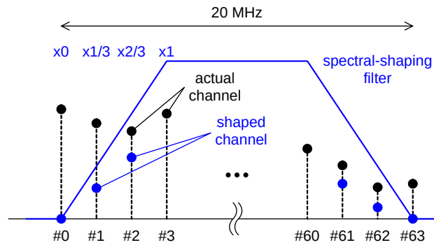
Figure 4.26: Spectral shaping (amplitudes of the outer three channels in each of lower and upper bands are multiplied by corresponding coefficients).
