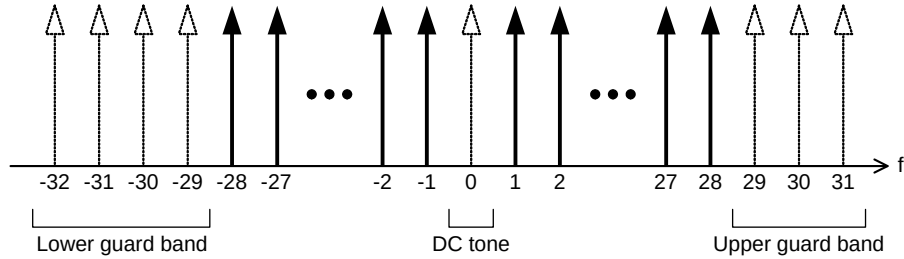
Figure 5.12: Subcarrier arrangement.
