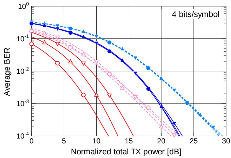
(b) TX-y/RX-y
