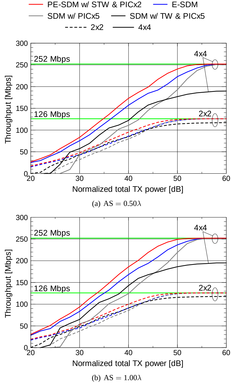
Figure 6.8: Throughput performance in the case of TX-x/RX-x array orientation in the LOS scenario (estimated CSI).
