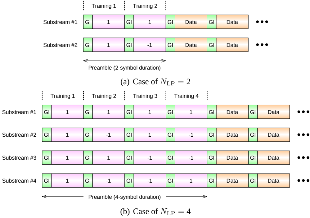
Figure 5.7: Frame formats.
