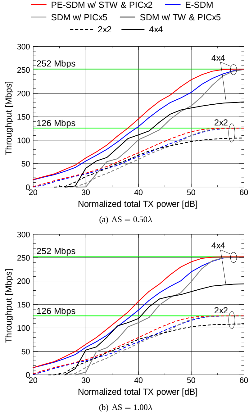
Figure 6.10: Throughput performance in the case of TX-x/RX-x array orientation in the NLOS scenario (estimated CSI).
