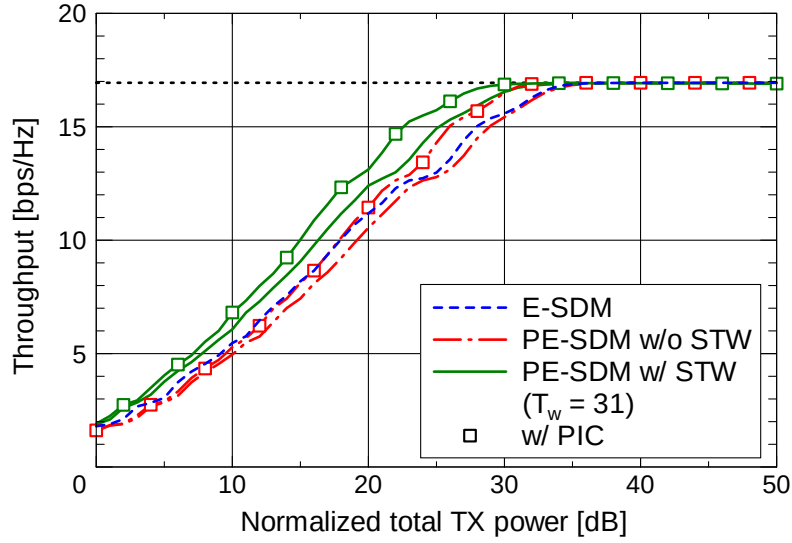
Figure 5.24: Throughput performance for the estimated CSI case.
