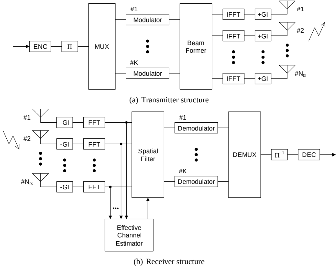
Figure 5.11: Block diagram.
