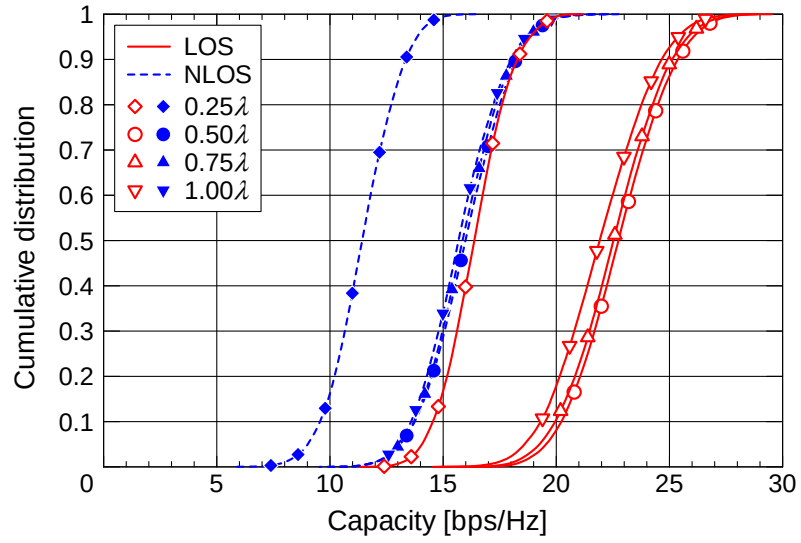
(b) TX-y/RX-y
