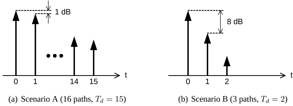
Figure 5.1: Two multipath fading scenarios.
