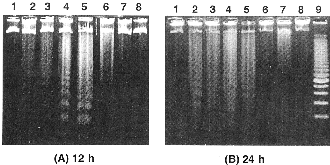
Fig. 3. Agarose gel electrophoresis of DNA in HL-60 cells treated with carotenoids and retinoic acid. HL-60 cells ( 1 \times 10^5 cells/ml) were incubated for 12 h (A) and 24 h (B) with the following agents: lane 1: ethanol, lane 2: fucoxanthin 4.5 \mu\text{M} , lane 3: fucoxanthin 11.3 \mu\text{M} , lane 4: fucoxanthin 22.6 \mu\text{M} , lane 5: camptothecin 100 \text{ nM} , lane 6: \beta -carotene 22.6 \mu\text{M} , lane 7: tetrahydrofuran, lane 8: retinoic acid 22.6 \mu\text{M} , lane 9: DNA size marker ( \times 180 \text{ bp} ).
