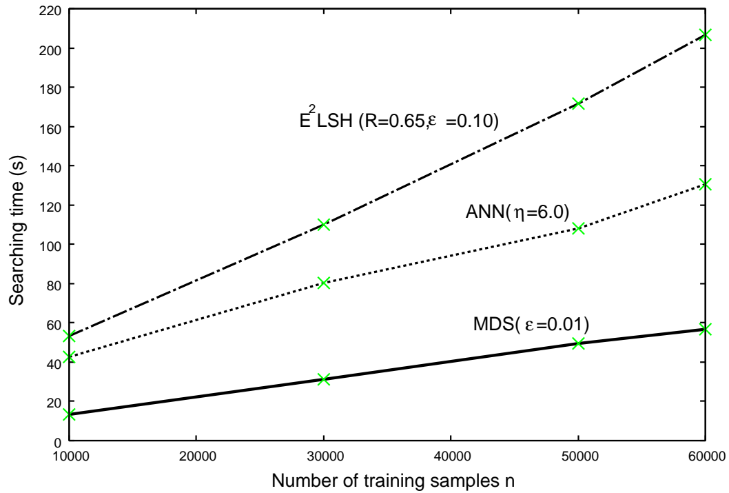
Fig. 5. Time complexity in data size.
