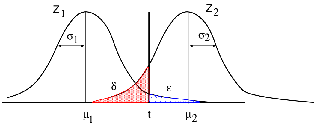
Fig. 7. Two densities causing two kinds of error.
