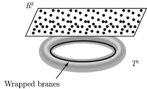
FIG. 1. Wrapped brane gases can be seen as point particles on three dimensions. Those point particles decay as the pressureless dust with e^{-3A(t)} .
