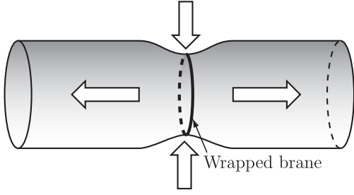
FIG. 2. A cycle where branes wrap is bound by the tension of branes. Cycles where branes do not wrap are stretched like a rubber tube in the four-dimensional Einstein frame. The cycles are homogeneously bound under the brane gas approximation, although this figure shows one of branes as an example.
