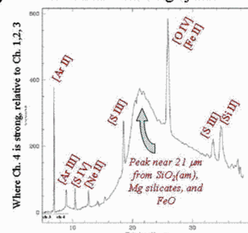
B Dust and gas from shocked O- and Si- burning ejecta
