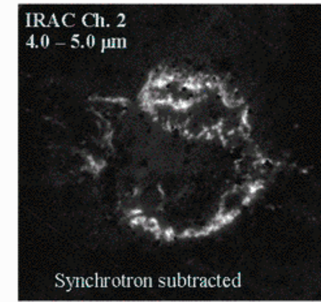
C Dust and gas primarily from shocked C-burning ejecta
