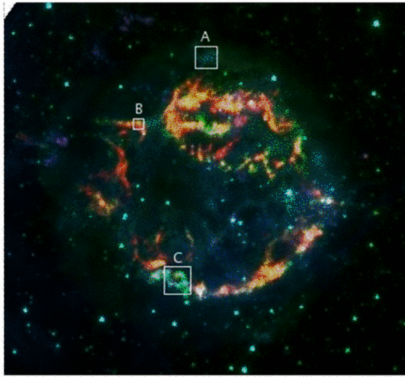
ABOVE: Color composite of IRAC Channels 4 (red), 2 (green) and 3 (blue). Emission is seen throughout the remnant in all IRAC bands. However, the relative strength in each band varies considerably across the remnant. The three labeled regions (A, B, C) correspond to the broadband IRS spectra shown at right. A: Ch. 1 relatively strong; B: Ch. 4 relatively strong; C: Ch. 2 & 3 relatively strong.
