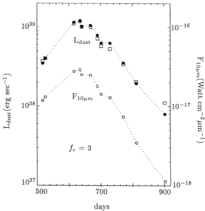
Fig. 8b. The same as Fig. 8a but for the clumpy ejecta of f_c = 3 . Up to \sim day 550 the total infrared luminosity attributes to the thermal radiation from \text{Al}_2\text{O}_3 grains, and afterwards the thermal radiation from \text{MgSiO}_3 grain dominates the total infrared luminosity, which is also true for Fig. 8a
