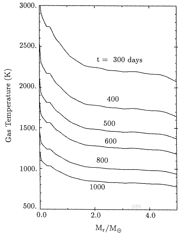
Fig. 3. The gas temperature distribution in the ejecta with \gamma = 1.27 at the given times after the explosion
