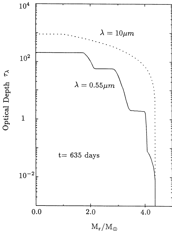
Fig. 7. The optical depths due to dust grains measured from the surface of grain formation region at day 635; the solid curve for \tau_{0.55} and the dotted curve for \tau_{10}
