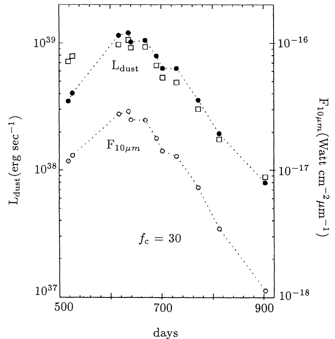
Fig. 9. The calculated infrared light curve for f_c = 30 . The disagreement between the observed total infrared luminosity and the calculated one is most remarkable for the optically thin ejecta at \lambda = 10\ \mu\text{m} around day 520. The reason is explained as the followings: When the ejecta is not extremely optically thick at \lambda = 10\ \mu\text{m} , the higher grain temperature is needed for larger f_c and smaller f_e to reproduce the observed 10\ \mu\text{m} flux. The resulting total infrared luminosity then becomes higher because the total infrared luminosity strongly depends on the grain temperature
