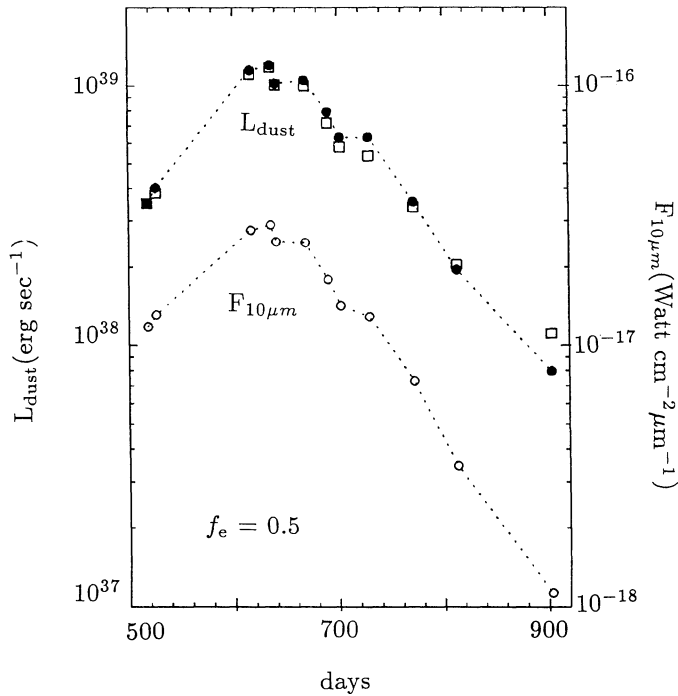
Fig. 8a. The comparison of the calculated total infrared light curve with the observed one for the condensation efficiency of f_e = 0.5 . The infrared luminosity is calculated from the condition that the calculated 10\ \mu\text{m} flux can reproduce the observed one. The open circles represent the observed 10\ \mu\text{m} flux, the filled circles the observed total infrared luminosity, and the open squares the calculated one
