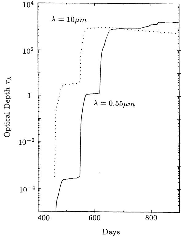
Fig. 6. The time evolution of the optical depths due to newly formed grains in the ejecta at the wavelengths of \lambda = 0.55 \mu\text{m} (solid curve) and 10 \mu\text{m} (dotted curve). The dust grain responsible for the optical depth is \text{Al}_2\text{O}_3 up to \sim day 550. The rapid increase of \tau_{10} starting at \sim day 550 is due to the condensation of \text{MgSiO}_3 grains, and the rapid increase of \tau_{0.55} starting at \sim day 620 is due to the condensation of \text{Fe}_3\text{O}_4 grains
