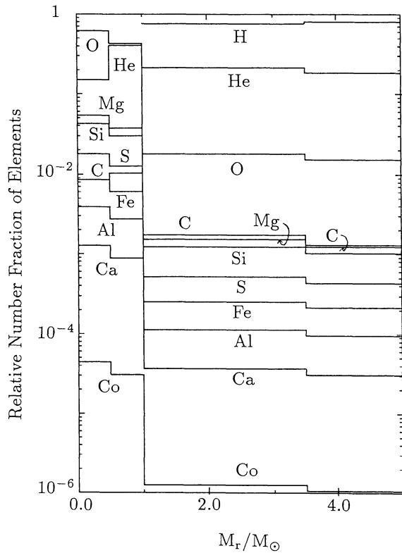
Fig. 1. The distribution of elements which are of interest to the grain formation in the ejecta at day 600 after the explosion, where the decay of ^{56}\text{Co} to ^{56}\text{Fe} is taken into account
