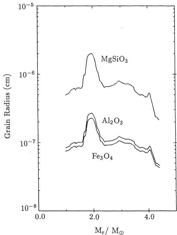
Fig. 5. The radii of dust grains formed in the region at 1.0 M_\odot \leq M_r \leq 4.4 M_\odot of the ejecta
