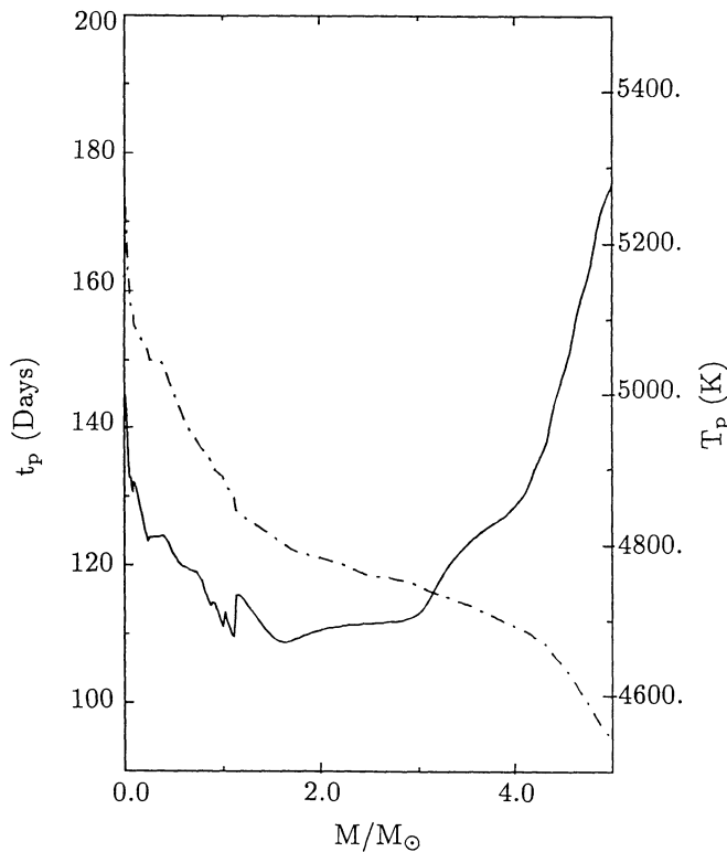
Fig. 2. The time t_p at which a gas passes through the photosphere and the gas temperature T_p at given locations in the ejecta. The dash-dotted curve is for t_p and the solid curve for T_p
