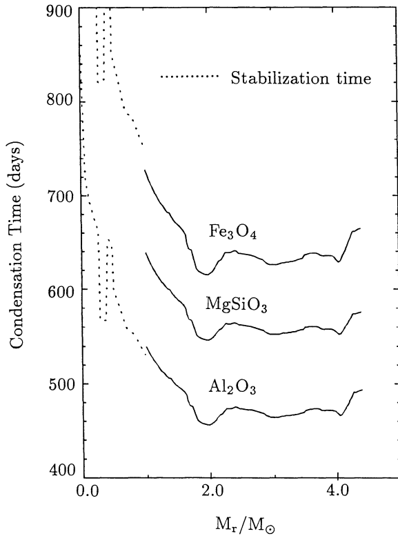
Fig. 4. The condensation time of each grain in the ejecta. The solid curves represent the condensation time determined by the process of homogeneous nucleation and grain growth, while the dotted curves represent the stabilization time of \text{Al}_2\text{O}_3 and \text{Fe}_3\text{O}_4 grains, after which dust grains grow stably against the heating due to the latent heat deposition during the grain growth
