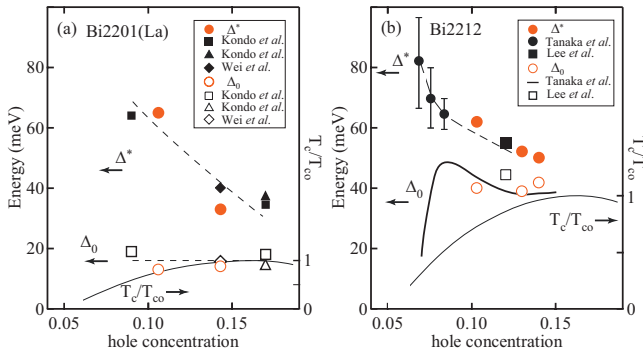
FIG. 7. (Color) (a) Doping-level dependence of \Delta^* (closed red circles) and \Delta_0 (open red circles) of Bi2201(La), plotted together with ARPES data \Delta_{\text{ARPES}}^* and \Delta_{\text{ARPES}}^0 reported by Kondo et al. (Ref. 9) (closed and open triangles), Kondo et al. (Ref. 18) (closed and open squares), and Wei et al. (Ref. 20) (closed and open rhombi). (b) Doping-level dependence of \Delta^* (closed red circles) and \Delta_0 (open red circles) of Bi2212, plotted together with ARPES data \Delta_{\text{ARPES}}^* and \Delta_{\text{ARPES}}^0 reported by Tanaka et al. (Ref. 8) (closed black circles and solid line) and Lee et al. (Ref. 16) (closed and open squares). The scale for T_c (the right-hand axis) is normalized by the optimal value of the critical temperature T_{c0} .
