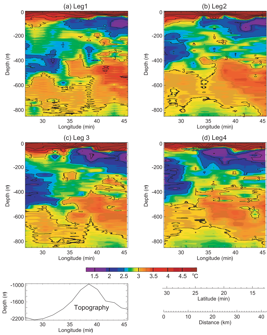
Figure 3: Vertical sections of potential temperature and the bottom topography along the observation line. Contour intervals are 0.5\text{ }^{\circ}\text{C} for \leq 3^{\circ}\text{C} and 1^{\circ}\text{C} for > 3^{\circ}\text{C} . The North Pacific Ocean (the Sea of Okhotsk) is on the right (left) hand side.
