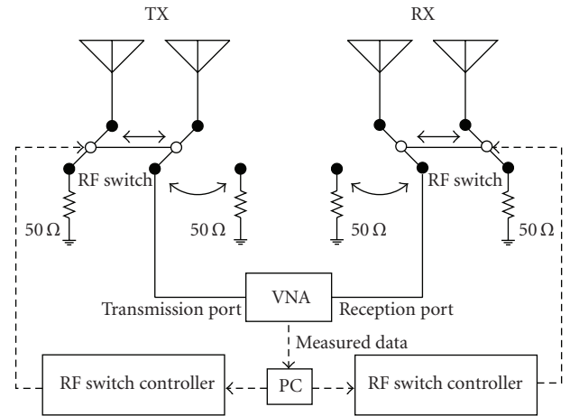
FIGURE 2: Channel measurement system.
