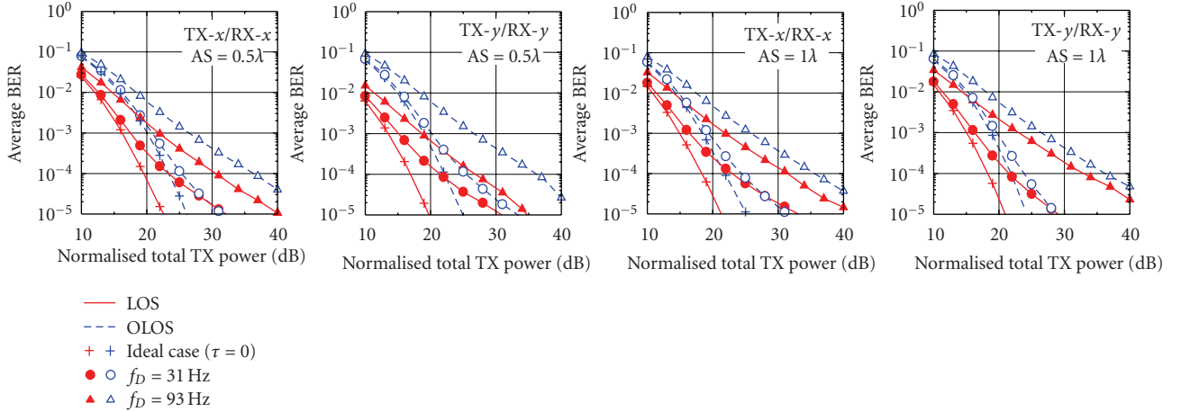
FIGURE 16: Uplink and downlink MIMO positions for the different f_D .
