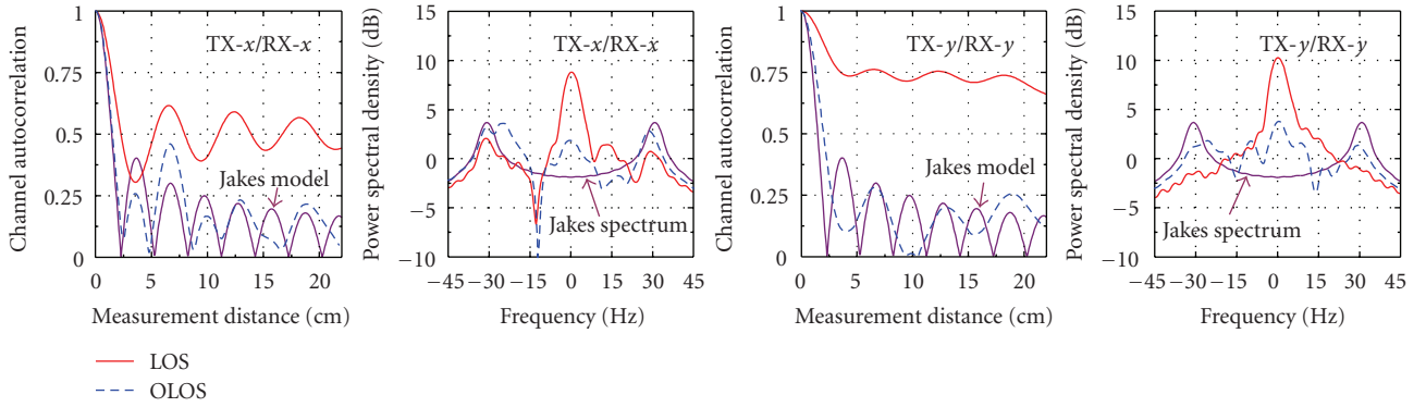
(b) RX array motion along the y-axis and AS = 0.5\lambda
