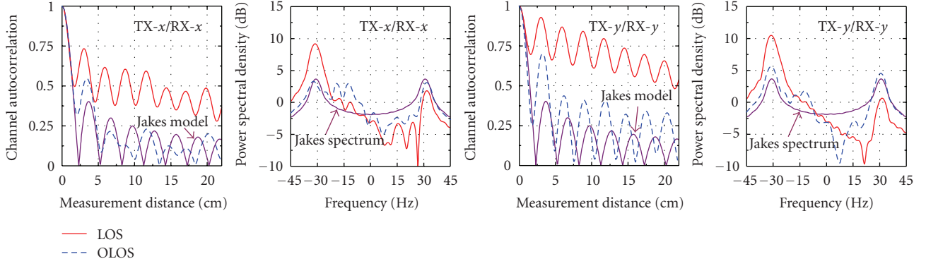
(a) RX array motion along the x-axis and AS = 0.5\lambda
