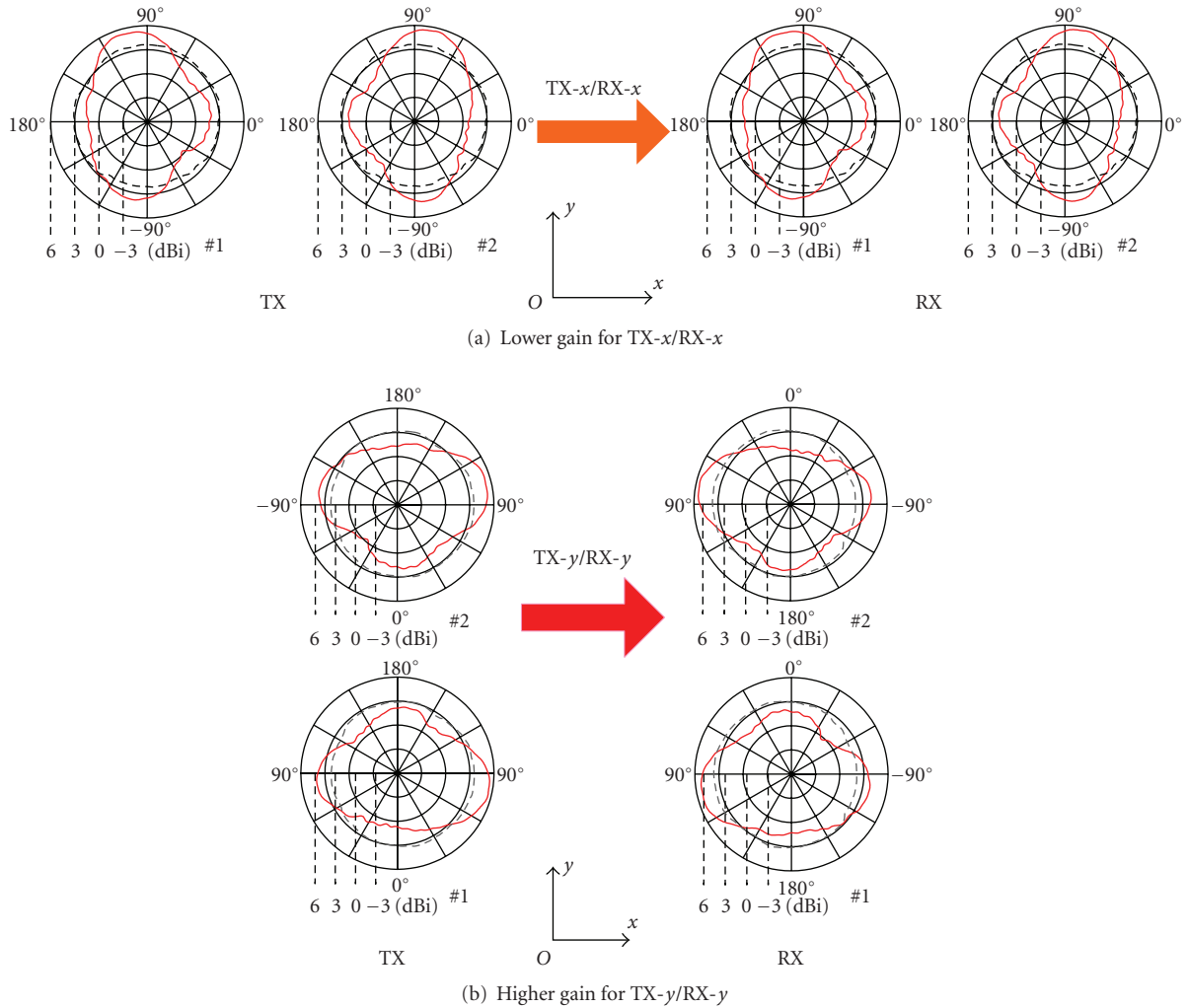
FIGURE 6: Antenna gain toward the direct wave for the case of AS = 0.5\lambda .
