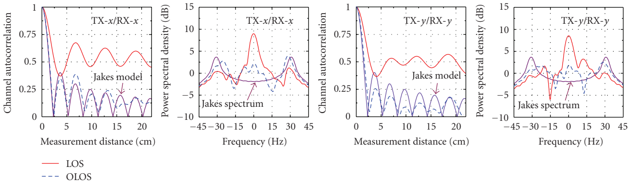
(d) RX array motion along the y-axis and AS = 1.0\lambda
