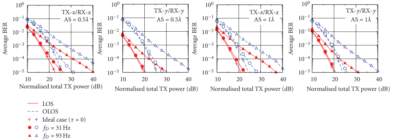
FIGURE 17: BER performance of 2 \times 2 MIMO E-SDM system.
