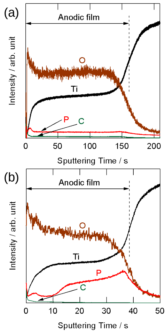
Fig. 4 GDOES depth profiles of the anodic films formed on titanium at (a) 5 V and (b) 20 V in 0.6 \text{ mol dm}^{-3} \text{ K}_2\text{HPO}_4 + 0.2 \text{ mol dm}^{-3} \text{ K}_3\text{PO}_4 glycerol electrolyte containing 0.04 mass% water at 433 K for 3.6 ks.
