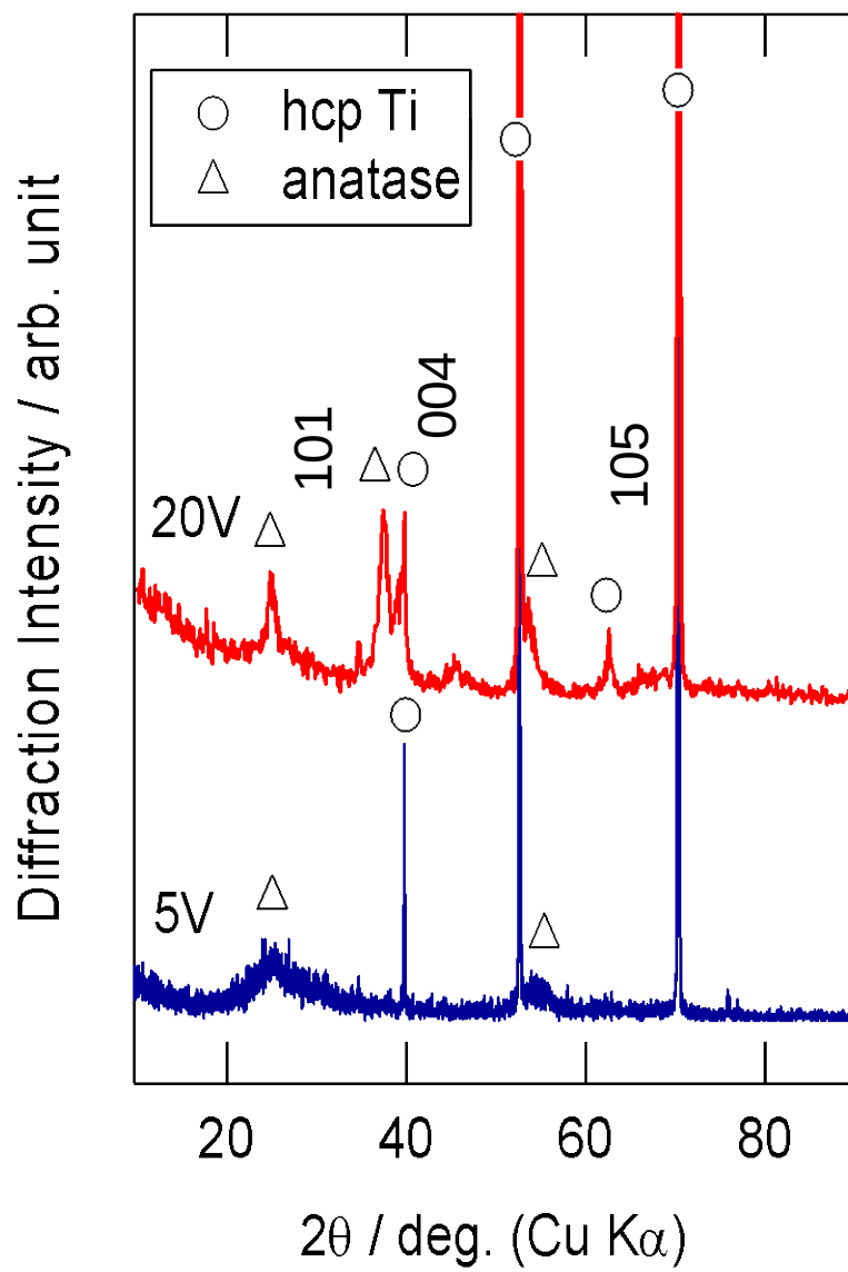
Fig. 6 X-ray diffraction patterns of titanium specimens anodized at 5 and 20 V in 0.6 \text{ mol dm}^{-3} \text{ K}_2\text{HPO}_4 + 0.2 \text{ mol dm}^{-3} \text{ K}_3\text{PO}_4 glycerol electrolyte containing 0.04 mass% water at 433 K for 3.6 ks.
