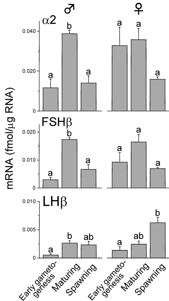
Fig. 2. Changes in the amounts of GTH subunit mRNAs during sexual maturation. The amounts of GTH subunit mRNAs in the control cell cultures on day 0 are indicated ( n=4-6 ). Values with different characters are significantly different among reproductive stages ( P < 0.05 ).
