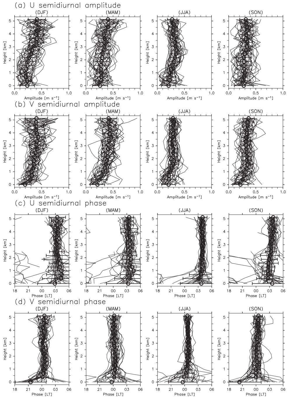
Fig. 14. As for Fig. 6, but for the semidiurnal wind component. For (c) and (d), data are not plotted in the case that SE exceeds 6 hr.
