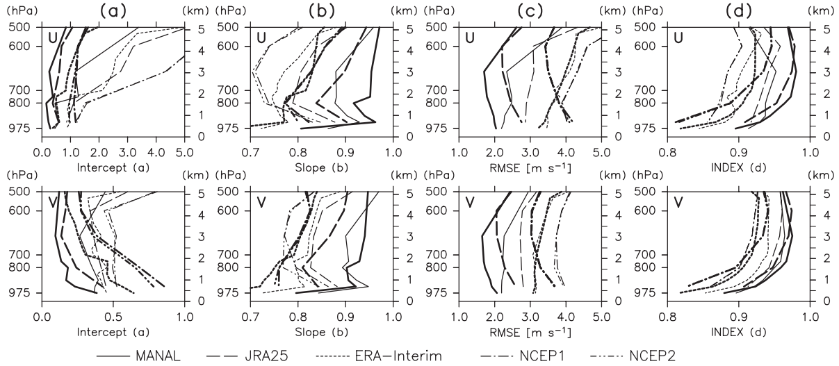
Fig. 2. Vertical profiles of the (a) intercept and (b) slope of the least-squares regression, (c) RMSE, and (d) index of agreement, for (top) the zonal wind component and (bottom) the meridional wind component, with respect to WINDAS data. Solid lines are for MANAL1, dashed lines for JRA25, dotted lines for ERA-Interim, dot-dashed lines for NCEP1, and dot-dot-dashed lines for NCEP2. Thick (thin) lines are for JJA (DJF). The correspondence between pressure levels and height levels follows that described in Table 1. See the text for details.
