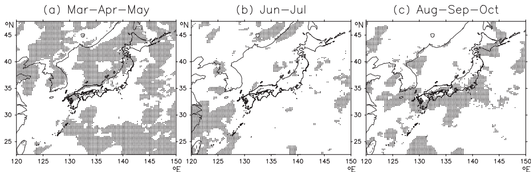
Fig. 9. Regions and time periods for which the diurnal amplitude of v attains a maximum at 800 hPa derived from MANAL1 data. Panel (a) shows such regions (dotted) in March–May, panel (b) in June–July, and panel (c) in August–October.
