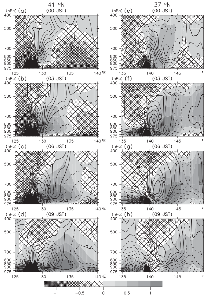
Fig. 13. Longitude–pressure distributions of the diurnal component of v (contours) and Z (gray scale), as derived from MANAL1 data at (a) 00 JST, (b) 03 JST, (c) 06 JST, and (d) 09 JST along 41°N between 125°E and 140°E, and at (e) 00 JST, (f) 03 JST, (g) 06 JST, and (h) 09 JST along 37°N between 135°E and 150°E, in August–September–October (ASO). Black shading indicates the topography. Three-hourly data were compiled from the harmonic diurnal component (see Section 2).
