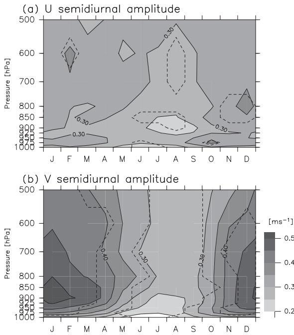
Fig. 8. As for Fig. 5, but for the semidiurnal amplitudes from MANAL2.
