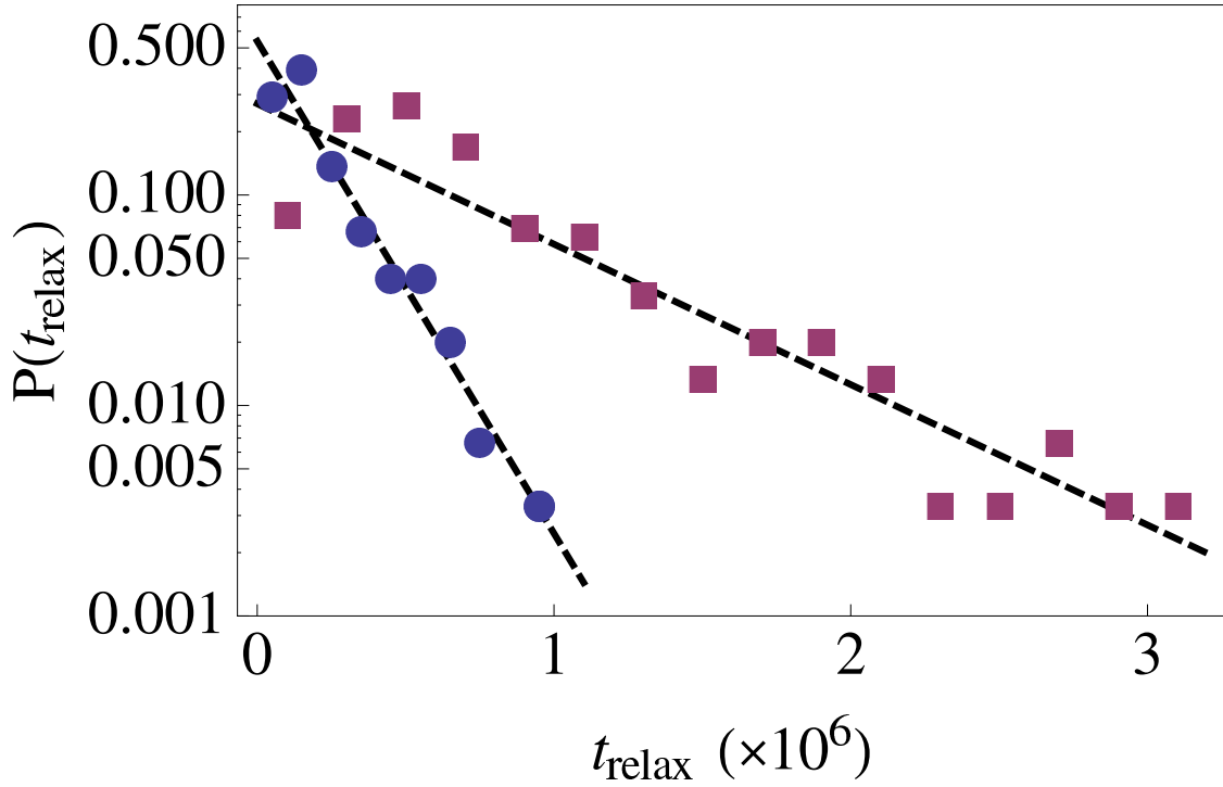
Figure 7. Distribution of t_{\text{relax}} for k = 100 (blue circles) and k = 200 (red squares). The initial conditions are x_i = i - (N + 1)/2 , y_i = 0 , p_i^x = \xi_i^{(x)} for 1 \leq i \leq N , and p_1^y = 0.1 + \xi_1^{(y)} , p_i^y = \xi_i^{(y)} ( 2 \leq i \leq N ), where \xi_i^{(x)} and \xi_i^{(y)} ( i = 1, \dots, N ) are independent random numbers uniformly distributed over the interval [0, 10^{-8}] . For each value of k , the numbers of samples are 200 and the system size is N = 6 . Both distributions are shown on a semi-log scale. The dashed lines show P(t_{\text{relax}}) = c \exp(-\alpha t_{\text{relax}}) . For k = 100 , c = 0.544 and \alpha = 5.39 \times 10^{-6} . For k = 200 , c = 0.271 and \alpha = 1.54 \times 10^{-6} .
