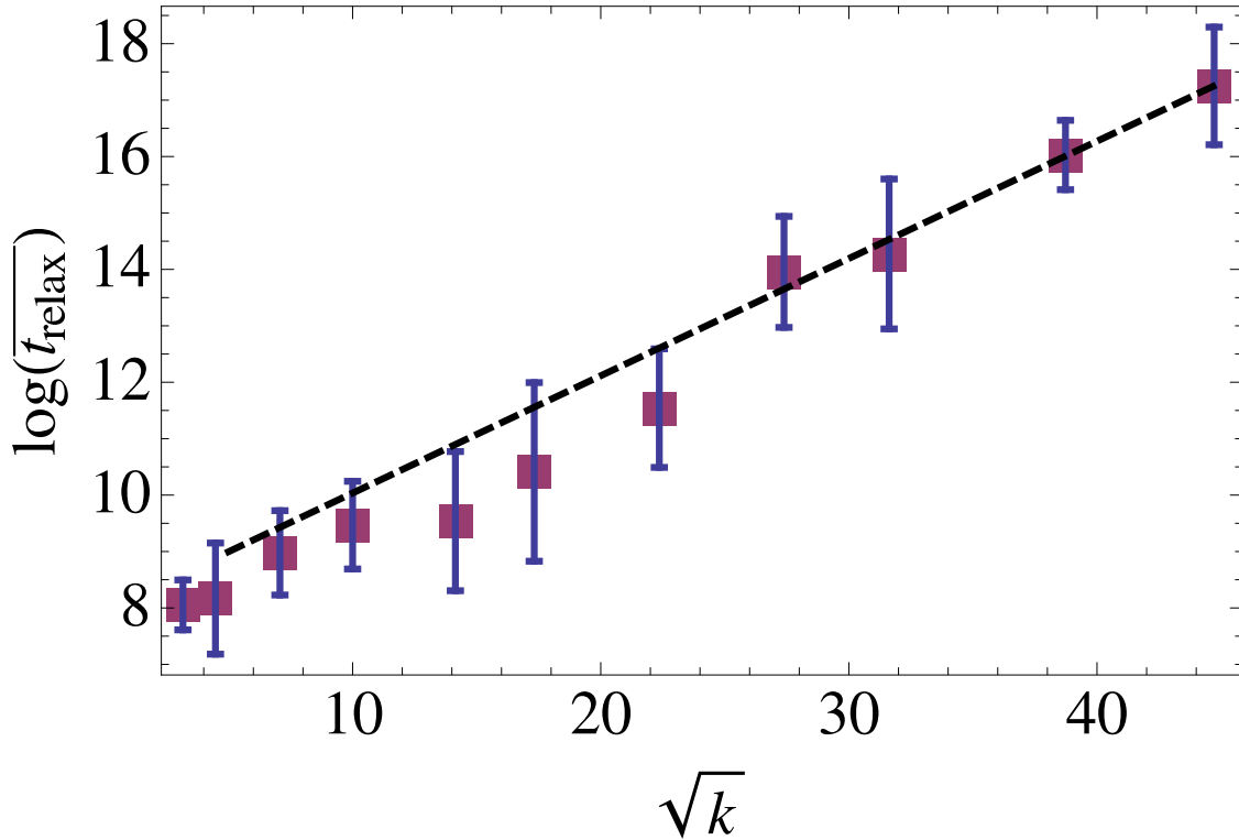
Figure 6. k dependence of average relaxation time t_{\text{relax}} . At each k value, 15 samples are taken. The system size is N = 6 . Threshold value \Delta_0 = 10^{-7} . The time step \delta t of integration is scaled as \delta t = 0.125 \times \sqrt{10}/\sqrt{k} . The initial conditions are x_i = i - (N + 1)/2 , y_i = 0 , p_i^x = \xi_i^{(x)} for 1 \leq i \leq N , and p_1^y = 0.1 + \xi_1^{(y)} , p_i^y = \xi_i^{(y)} ( 2 \leq i \leq N ), where \xi_i^{(x)} and \xi_i^{(y)} ( i = 1, \dots, N ) are independent random numbers uniformly distributed over the interval [0, 10^{-8}] . The error bars represent standard deviations of t_{\text{relax}}^{(\text{sample})} for 15 samples. The dashed line shows t_{\text{relax}} = 5.52 \times 10^4 \exp(0.415\sqrt{k}) obtained by fitting.
