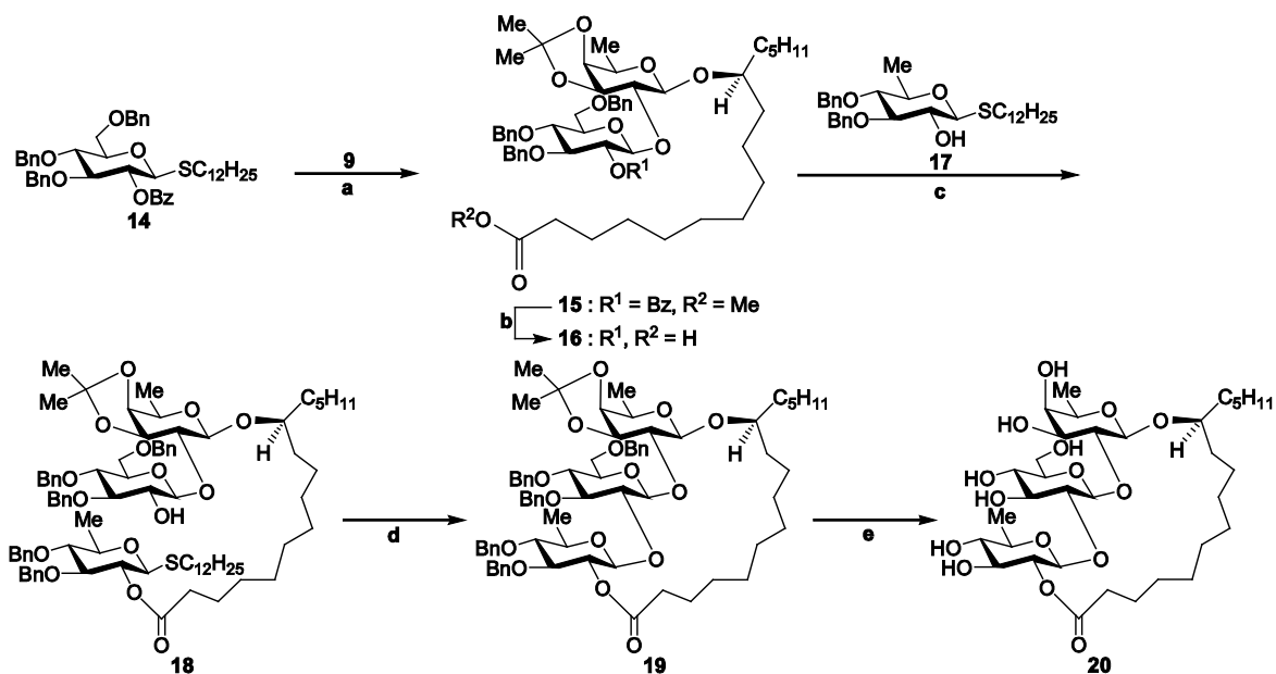
Scheme 3 Total synthesis of tricolorin F. Reagents and conditions: (a) MeOTf, MS 4 Å, CH 2 Cl 2 , r.t., 6 h, 83%; (b) NaOH, THF–EtOH, 50 °C, 4 h, 99%; (c) WSC · HCl, DMAP, CH 2 Cl 2 , r.t., 24 h, 72%; (d) MeOTf, MS 4 Å, CH 2 Cl 2 , r.t., 24 h, 70%; (e) i) HCl, MeOH, r.t., 2 h; ii) Pd/C, H 2 , MeOH, r.t., 24 h, 99%.
