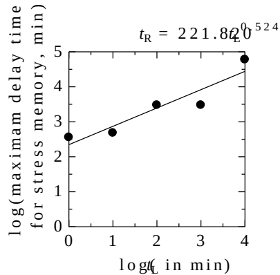
Fig. 2 Maximum delay time for stress memory with duration of load application t_L for Shirahama sandstone [1].
