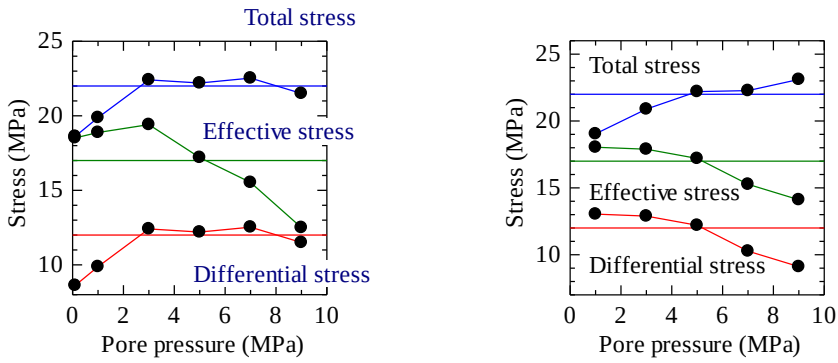
(a) Constant total confining pressure of 10 MPa
