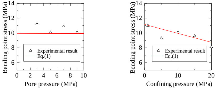
(a) Constant confining pressure of 10 MPa (b) Nearly constant pore pressure of 5 MPa Fig. 9 Bending point stress by uniaxial cyclic loading for triaxially preloaded saturated Kimachi sandstone. Preloaded differential axial stress was 12 MPa for all specimens. Preloaded pore pressure was 0.9 MPa and 4.9 MPa for confining pressure of 1 MPa and 5 MPa, respectively in (b).
