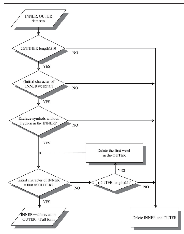
Fig. 2 Flow chart of the algorithm: conditional branch on INNER and OUTER.
