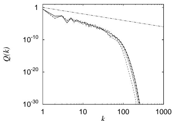
Figure 5. Time evolution of the spectra of active scalar at t = 70 (solid), 80 (dashed), 90 (dotted), and 100 (short-sashed) for \alpha = 0.4 , \nu = 1.0 \times 10^{-3} . The straight line has a slope of -2 .
