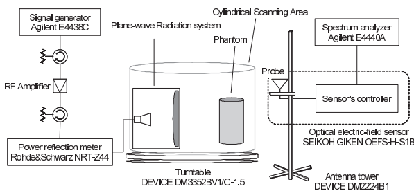
Fig. 5 Block diagram of the proposed experimental set-up for WB-SAR estimation.
