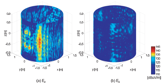
Fig. 12 Measured electric field distributions with the male adult phantom on cylindrical scanning area.
