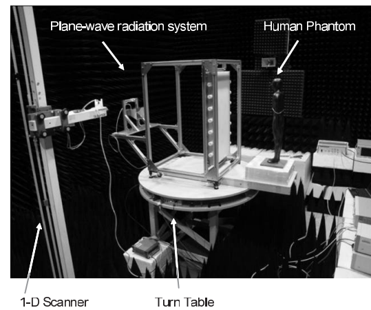
Fig. 10 Proposed experimental set-up in anechoic chamber.
