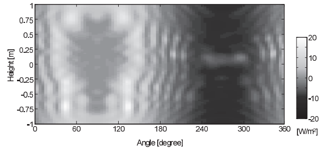
Fig. 4 Poynting vector (component of P_r ) distribution on the cylindrical surface for homogeneous male adult phantom.
