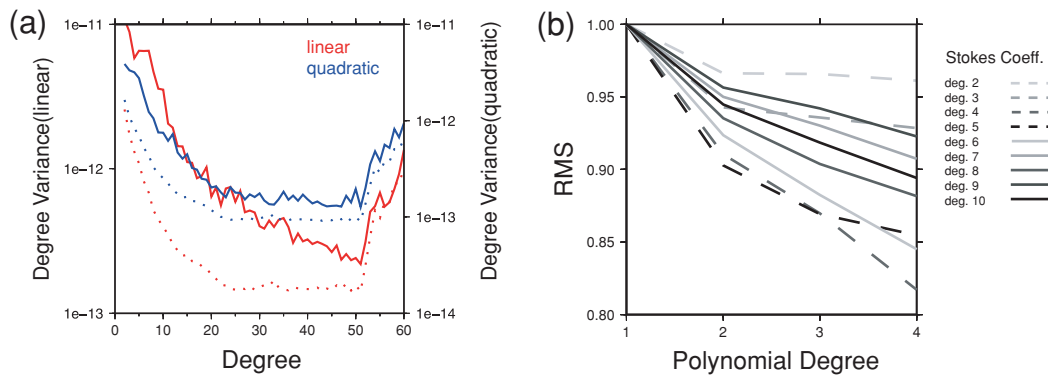
Figure 2. (a) Degree variance of linear and quadratic changes of GRACE TVG. Red and blue curves show linear and quadratic terms, respectively. They all exceed one-sigma errors shown with dotted curves. (b) Relationship between post-fit rms residuals of the Stokes coefficients of various spatial degrees and the polynomial degree for the assumed interannual fit (plus the seasonal terms). Residual decreases notably by adding the quadratic term (i.e. by changing polynomial degree from 1 to 2).
