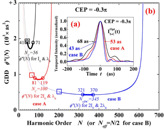
Fig. 10. (Color online) (a) Normalized pulse profile I_{S-C}^{\text{opt}}(t) after the optimum selection; (b) N -dependent GDD \phi''_{S-C}(N) curves at the pump intensity I_{\text{pump}} = I_0 , the pump wavelength \lambda_{\text{pump}} = \lambda_0 , and CEP = -0.3\pi : black curve for the intensity ( I_0 ) and wavelength ( \lambda_0 ) pump case, red curve for the double-intensity ( 2I_0 ) and wavelength ( \lambda_0 ) pump case, and blue curve for the double-intensity ( 2I_0 ), double-wavelength ( 2\lambda_0 ) pump case; ( N_{\text{eff}} = N/2 ). The open square ( \square ) and open circle ( \circ ) show the ends of upper branch and the ends of optimum region, respectively.
