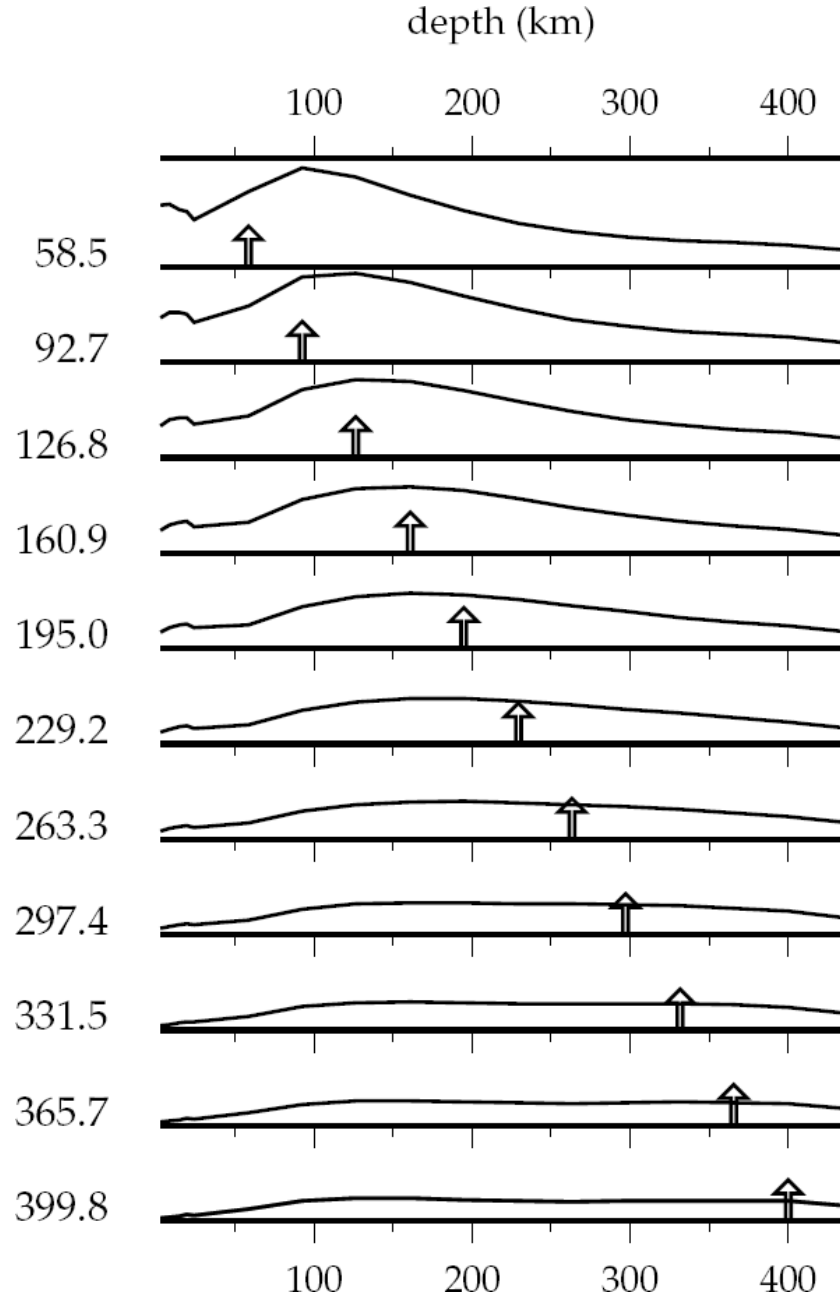
Figure 9: Resolution kernels for S-wave velocity profile beneath the location at (35 °N, 140°E). An ideal vertical resolution would show a delta-like peak around each depth marked by arrows. In this example, the structure is relatively well resolved down to 200-250 km in depth, mainly due to the fundamental mode sensitivity.
