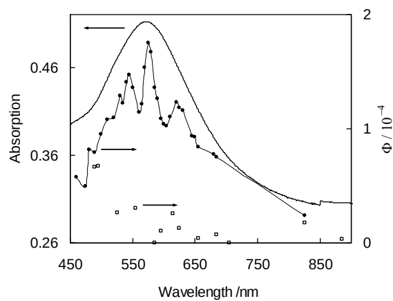
Fig. 9. Action spectrum of 2-propanol oxidation on \text{TiO}_2 (ST41): ● Au-modified, □ bare, and — absorption spectrum of \text{Au/TiO}_2 (ST41) measured with barium sulfate as a reference.
