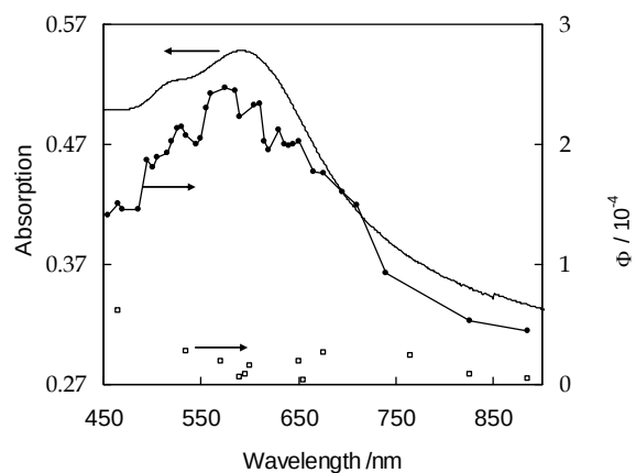
Fig. 8. Action spectrum of 2-propanol oxidation on \text{TiO}_2 (Aldrich_r): ● Au-modified, □ bare, and — absorption spectrum of \text{Au/TiO}_2 (Aldrich_r) measured with barium sulfate as a reference. 13d
