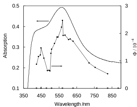
Fig. 10. Action spectrum of 2-propanol oxidation on \text{TiO}_2 (Aldrich_a): ● Au-modified, □ bare, and — absorption spectrum of \text{Au/TiO}_2 (Aldrich_a) measured with bare Aldrich_a as a reference.
