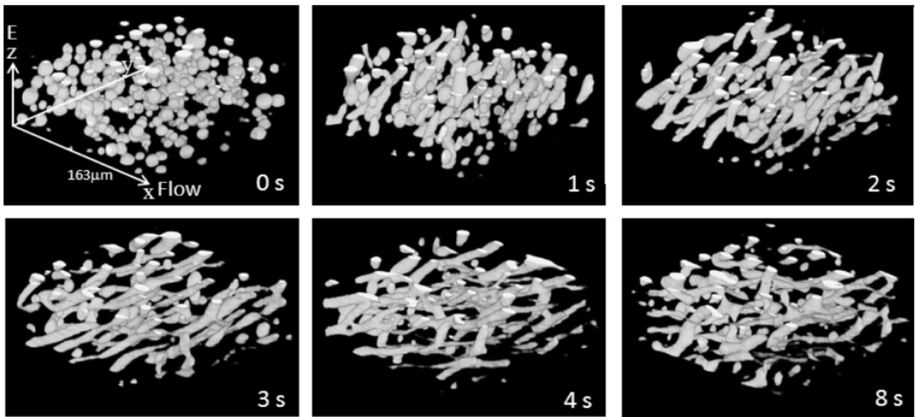
FIG. 4. 3D images in transient process, where the x , y , and z axes are taken along the flow, vorticity, and velocity gradient (the electric field) directions, respectively. The corresponding movie is provided in Ref. [21].
