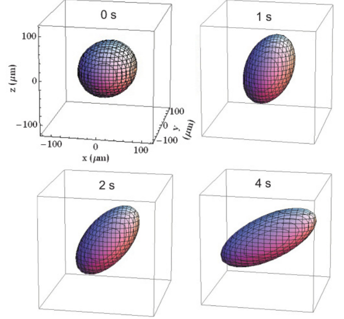
FIG. 6. (Color online) Time evolution of the ellipsoid corresponding to that of the surface tensor in Figs. 3 and 5. The corresponding movie is provided in Ref. [22].
