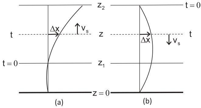
FIG. 13. (a) Upward scan and (b) downward scan, where the focal plane is located at z and v_s is the scan speed.
