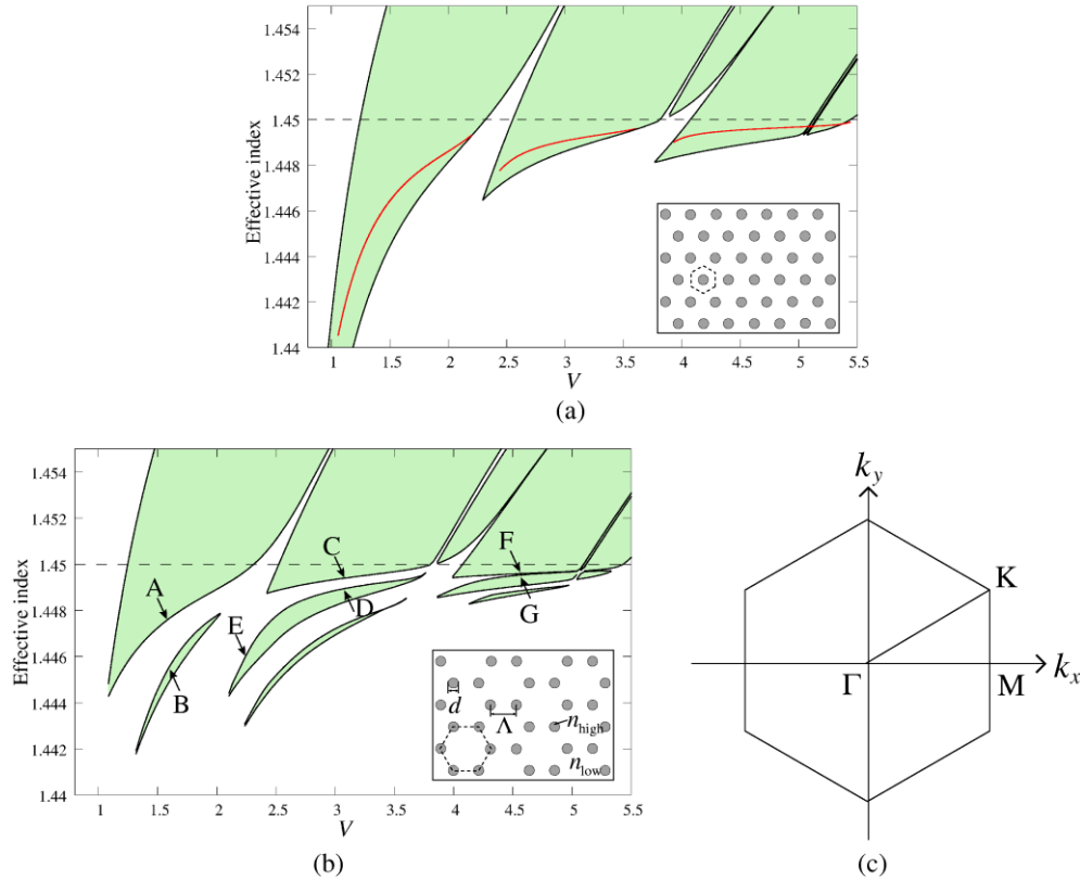
Fig. 7. Photonic band diagrams (green region) for the (a) triangular lattice and (b) honeycomb lattice for first, second, and third-order PBGs (from left to right), where red curves in (a) are dispersion curves of the fundamental-like mode for the 1-cell-core all-solid PBGF shown in Fig. 1(a) and the arrows in (b) correspond to the condition at which Bloch states will be presented in Fig. 8. The insets in (a) and (b) depict the corresponding lattice structure, where the hexagonal region stands for the unit cell. (c) First Brillouin zone boundary in reciprocal lattice space for two-dimensional triangular lattice with the pitch \Lambda' , where (k_x, k_y) = (0, 0) at \Gamma point, (k_x, k_y) = (2\pi/\sqrt{3}\Lambda', 0) at M point, and (k_x, k_y) = (2\pi/\sqrt{3}\Lambda', 2\pi/3\Lambda') at K point, where \Lambda' = \sqrt{3}\Lambda .
