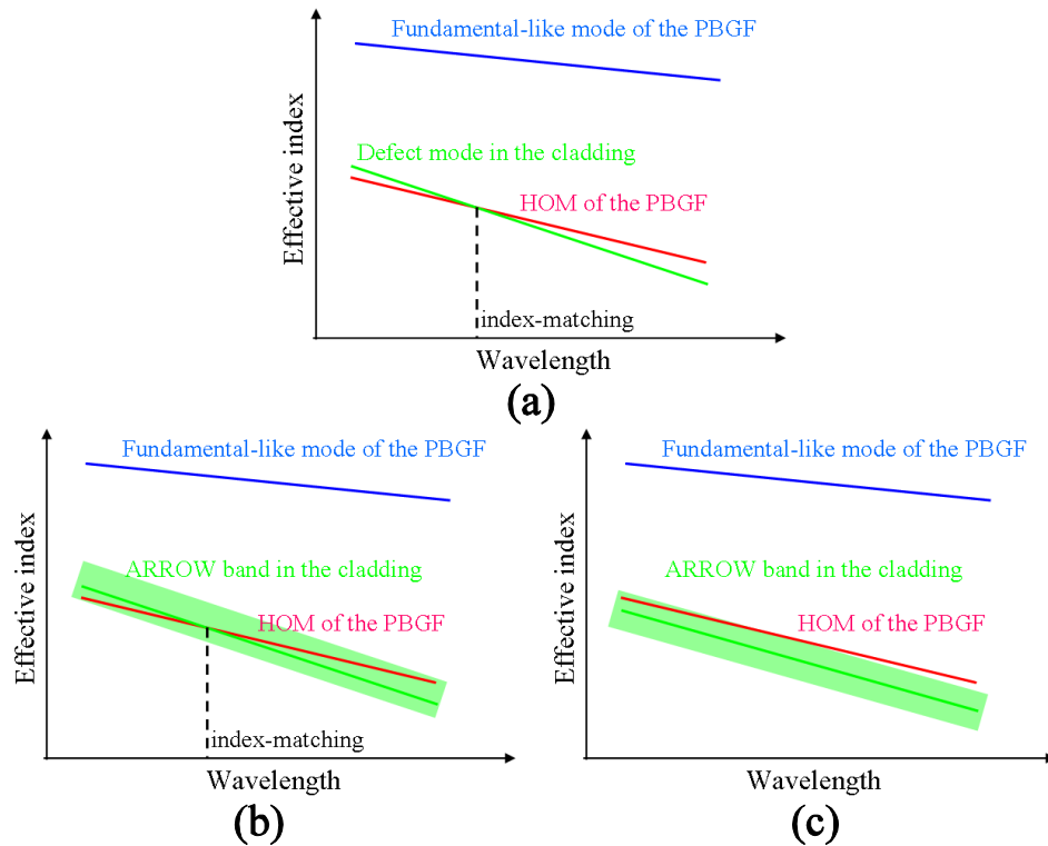
Fig. 3. Schematic representation of the dispersion relation for (a) the conventional HOM suppression method based on index-matching operating at only a particular wavelength that index-matching occurs, (b) the proposed method based on multiple resonant coupling operating for a wide wavelength range owing to photonic bands generated by ARROW modes in the cladding, and (c) the enhanced confinement loss mechanism which supports the HOM suppression at the condition that multiple resonant coupling does not occur.
