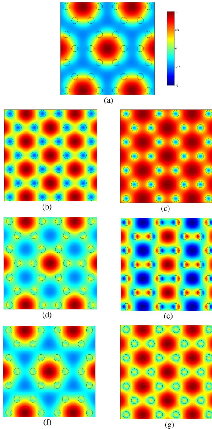
Fig. 8. One of the transverse electric field components ( E_x ) of Bloch states corresponding to the photonic bands' edge indicated by arrows from A to G in Fig. 7(b) is depicted from (a) to (g), respectively. The states of A, B, C, D, E, F, and G in Fig. 7(b) correspond to K, \Gamma , \Gamma , K, M, K, and \Gamma , respectively, and are composed of even state of LP_{11} rod modes, even state of LP_{02} rod modes, even state of LP_{02} rod modes, even state of LP_{12} rod modes, odd state of LP_{11} rod modes, even state of LP_{12} rod modes, and even state of LP_{03} rod modes, respectively.
