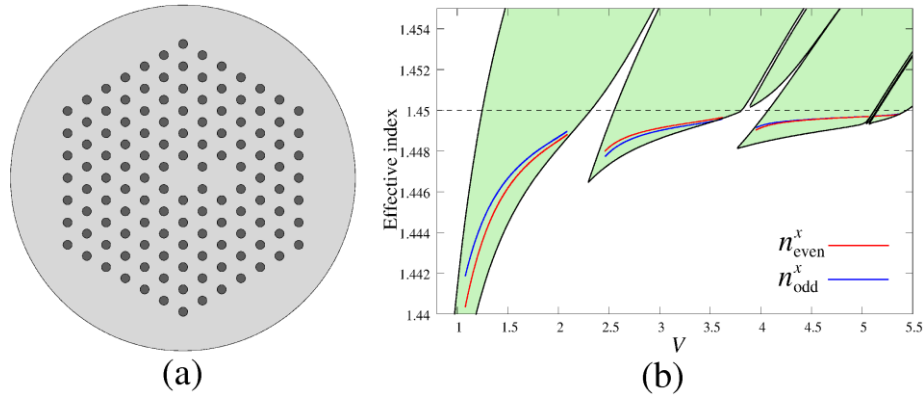
Fig. 9. (a) Cross section of conventional all-solid PBGF coupler with 2 cores. (b) Dispersion curves of the x-polarized even (red curves) and odd modes (blue curves) for the coupler, where the region with green represents the PBG of the triangular lattice for the first, second, and third-order PBGs (from left to right). Apparently, the effective index for the odd mode is larger in the odd-ordered PBGs.
