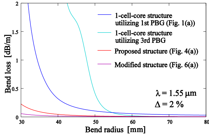
Fig. 5. Bending losses as function of bending radius at \lambda = 1.55 \mu\text{m} for the proposed structure shown in Fig. 4(a) (red curve) and modified structure shown in Fig. 6(a) (purple curve), where d/\Lambda = 0.5 and \Lambda = 5.6 \mu\text{m} . As a reference, results are also shown for conventional 1-cell-core structure with triangular lattice cladding utilizing the first-order PBG shown in Fig. 1(a) (blue curve), where d/\Lambda = 0.4 and \Lambda = 7.0 \mu\text{m} , and conventional 1-cell-core structure utilizing the third-order PBG (cyan curve). For the structure utilizing the third-order PBG, the parameters are chosen as d/\Lambda = 0.56 and \Lambda = 13.5 \mu\text{m} with 6 cladding rings.
