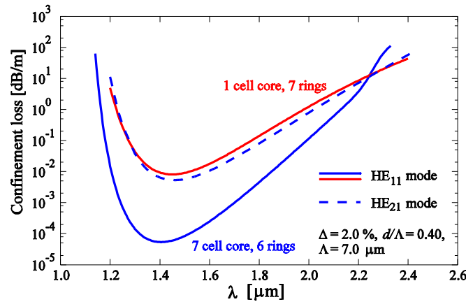
Fig. 2. Confinement losses as a function of wavelength for uniform 1-cell-core structure (red curve) and 7-cell-core structure (blue curves) in the first-order PBG. Exploiting the 7-cell-core structure in the first-order PBG also leads to the improvement of the confinement loss property as well as the bending loss property, while causing the multi-mode operation.
