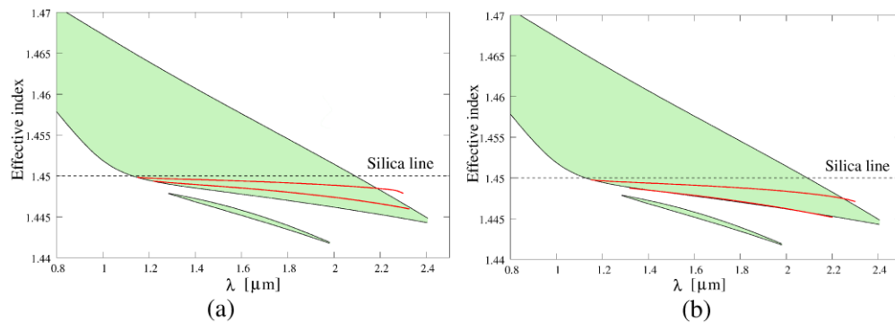
Fig. 11. (a) Dispersion curves of the fundamental-like and the HOM ( \text{HE}_{21} mode) for the (a) 2nd cladding fiber shown in Fig. 10(b), and (b) proposed fiber with the heterostructured cladding shown in Fig. 4(a) in the first-order PBG (red curves), where the green region stands for the PBG of honeycomb lattice.
