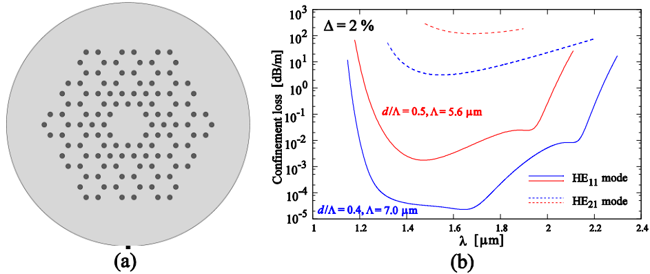
Fig. 4. (a) Cross section for the proposed all-solid PBGF which satisfies the multiple resonant coupling shown in Fig. 3(b) or enhanced confinement loss mechanism shown in Fig. 3(c). The cladding has periodically arranged multiple cores. (b) Confinement losses as a function of wavelength for the proposed structure with 6 cladding rings. The HOM is effectively suppressed while keeping the confinement loss low for the fundamental-like mode for d/\Lambda = 0.4 and \Lambda = 7.0 \mu\text{m} (blue curves), as well as for d/\Lambda = 0.5 and \Lambda = 5.6 \mu\text{m} (red curves).
