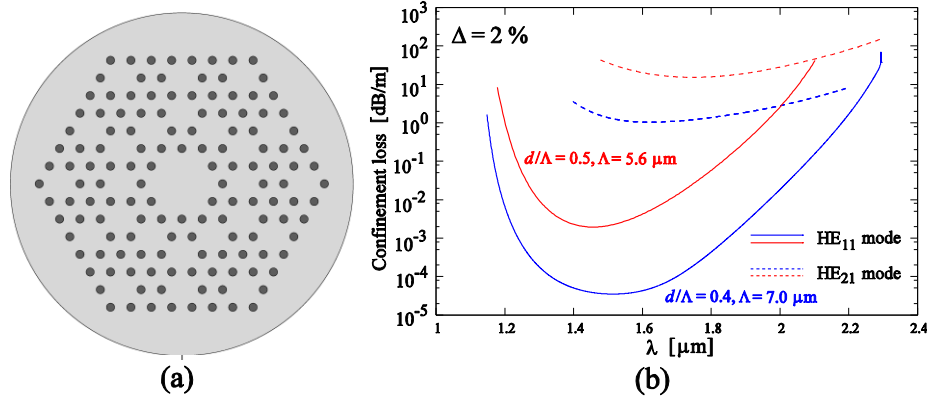
Fig. 6. (a) Cross section of the modified heterostructured PBGF, where the several high-index rods are embedded in the low-index regions designed as causing the multiple resonant coupling mechanism. (b) Confinement losses as a function of wavelength for the guided modes with 6 cladding rings. The HOM is effectively suppressed while keeping the confinement loss low for the fundamental-like mode for d/\Lambda = 0.4 and \Lambda = 7.0 \mu\text{m} (blue curves), as well as for d/\Lambda = 0.5 and \Lambda = 5.6 \mu\text{m} (red curves).
