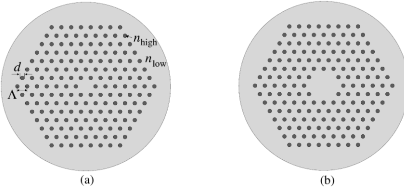
Fig. 1. Cross sections of typical all-solid PBGF ("uniform" structure) with (a) 1-cell core and 7 rings, and (b) 7-cell core with 6 rings (cladding region is in keeping with that of the fiber with 1-cell core and 7 rings), where d stands for diameter of high-index rods, \Lambda is the distance between adjacent rods, and n_{\text{high}} , n_{\text{low}} are refractive indices of high-index rods and low-index background, respectively. Unless the exceptional clause is shown, the structural parameters of d/\Lambda = 0.4 , \Lambda = 7.0 \mu\text{m} , n_{\text{high}} = 1.48 , and n_{\text{low}} = 1.45 are considered.
