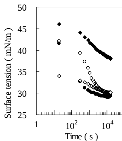
Figure 5. Time course of the water surface tension after the addition of LS, DAE0-AL (3), DAE0-KL (5), and DAE0-LS (1). The value in parenthesis is a charge ratio of epoxy compound (g) to LS (g). o, DAE0-LS(1); •, DAE0-KL(5); ◇, DAE0-AL(3); ♦, LS.
