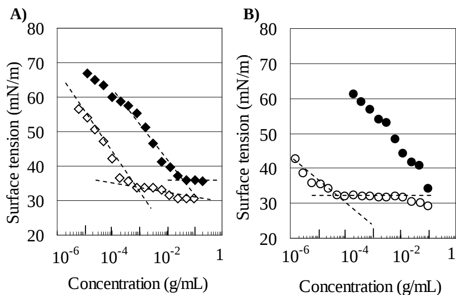
Figure 2. Surface tension-concentration isotherms for EPEG-AL, DAEO-AL, EPEG-KL, and DAEO-KL. A) \diamond , EPEG-AL(13,4); \blacklozenge , DAEO-AL(3); B) \bullet , EPEG-KL(13,6); \circ , DAEO-KL(5).
