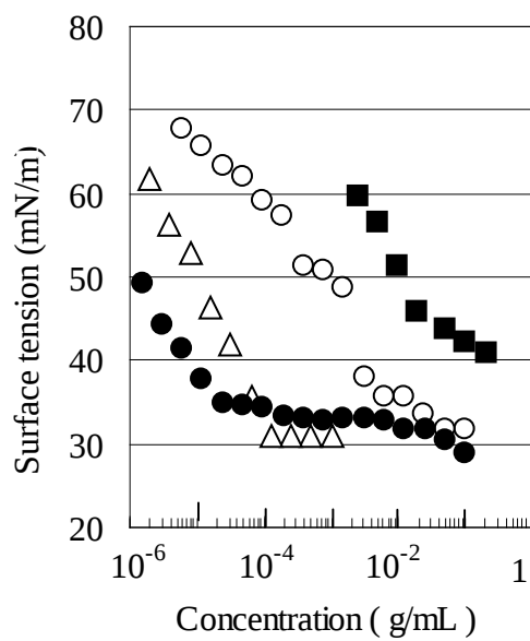
Figure 3. Surface tension-concentrations isotherms for LS, DAEO, and DAEO-LS. •, LS; ○, DAEO-LS(0.005); Δ, DAEO; ■, DAEO-LS (0.5).
