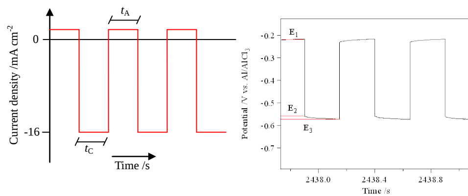
Fig. 9 Current pulse waveform for Al electrodeposition and potential response during BCP polarization.
