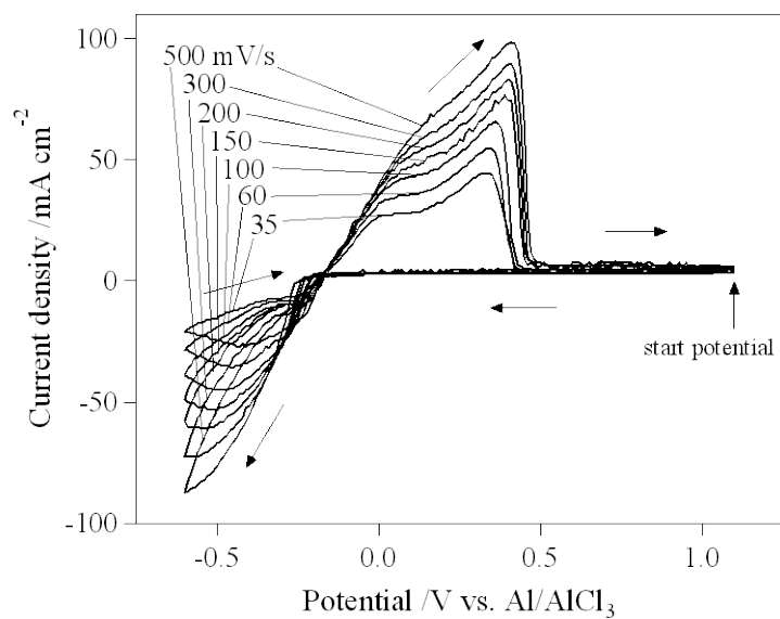
Fig. 1 Cyclic voltammograms of Pt in the [EMIm]Cl/AlCl 3 (0.5 mol%) plating bath measured with scan rates of 35, 60, 100, 150, 200, 300, and 500 mV s -1 .
