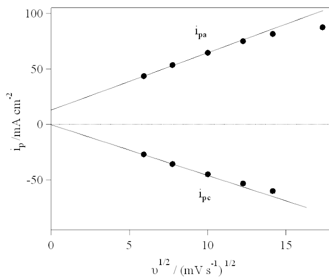
Fig. 2 Relationship between cathodic peak current ( i_{pc} ) and anodic peak current ( i_{pa} ) against square root of the scan rate ( v ) obtained from the data shown in Fig. 1.
