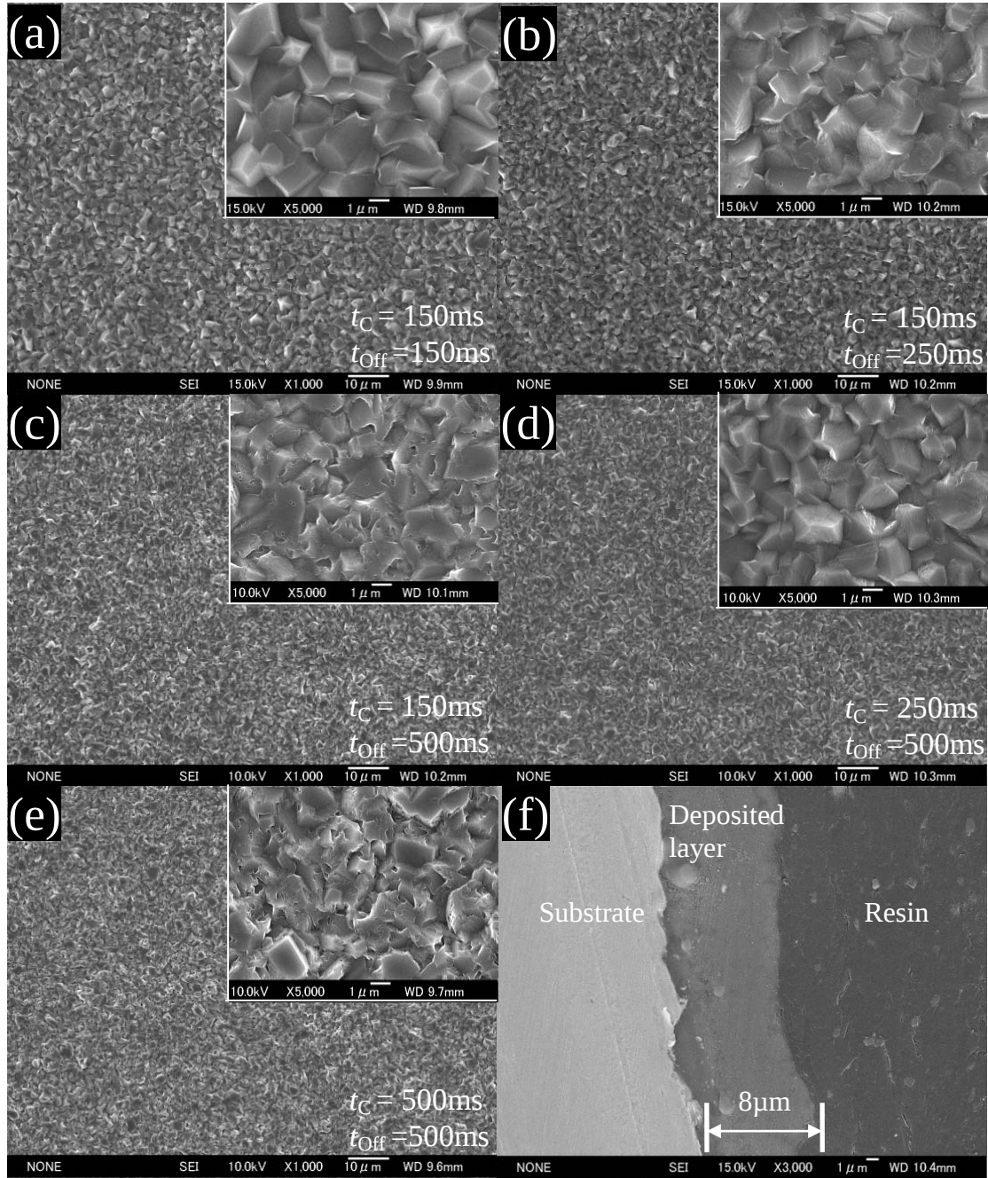
Fig. 8 SEM images of the Al surface electrodeposited from the [EMIm]Cl/AlCl 3 (0.5 mol%) bath using the MCP method at I_C = -16.0 \text{ mA cm}^{-2} . (a) r_C = 0.5 , f = 3.3 \text{ Hz} ; (b) r_C = 0.375 , f = 2.5 \text{ Hz} ; (c) r_C = 0.23 , f = 1.54 \text{ Hz} ; (d) r_C = 0.33 , f = 1.33 \text{ Hz} ; (e) r_C = 0.5 , f = 1 \text{ Hz} . (f) Cross-sectional SEM image of (c).
