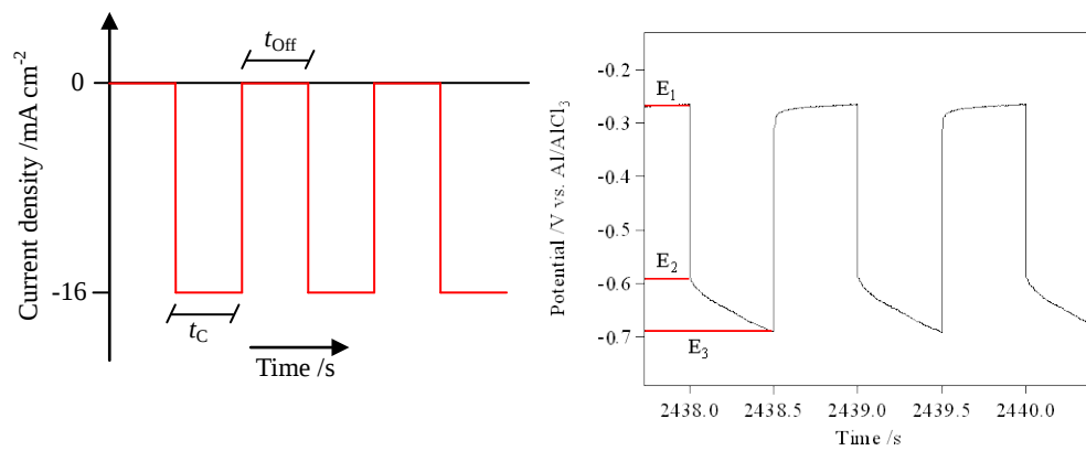
Fig. 7 Current pulse waveform for Al electrodeposition and potential response during MCP polarization.
