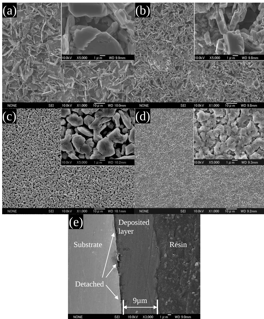
Fig. 6 SEM images of the Al surface electrodeposited from the [EMIm]Cl/AlCl 3 (0.5 mol%) bath using galvanostatic polarization at (a) -3.0 mA cm -2 , (b) -4.5 mA cm -2 , (c) -6.0 mA cm -2 , and (d) -8.0 mA cm -2 . (e) Cross-sectional SEM image of (d).
