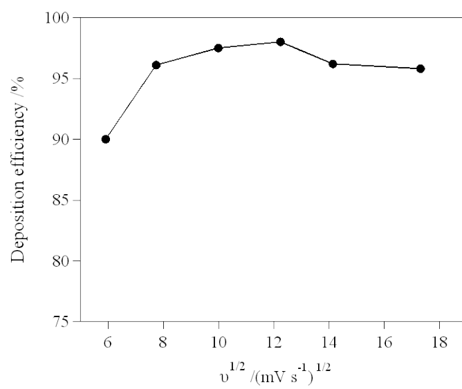
Fig. 3 Efficiency of Al electrodeposition against square root of the scan rate ( v ) during the potential scan shown in Fig. 1.
