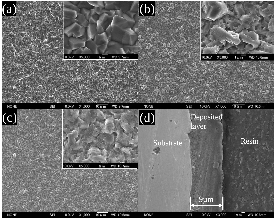
Fig. 10 SEM images of the Al surface electrodeposited from the [EMIm]Cl/ \text{AlCl}_3 (0.5 mol%) bath using the BCP method with duty ratio r_c = 0.5 , f = 2 Hz, cathodic current density I_c = -16 \text{ mA cm}^{-2} , and anodic current density I_a = (a) 0.3, (b) 0.5, and (c) 1.0 \text{ mA cm}^{-2} . (d) Cross-sectional SEM image of (c).
