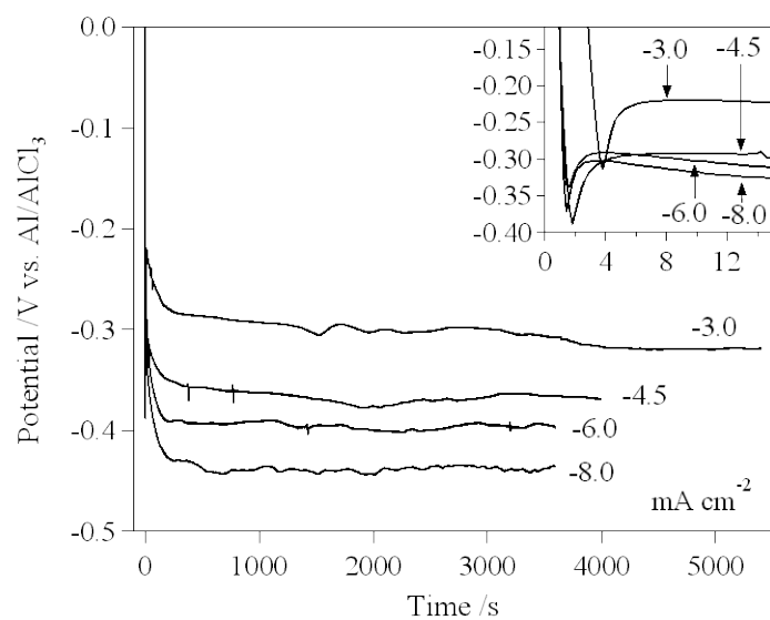
Fig. 5 Potential-time transition of Pt electrode during galvanostatic polarization for Al electrodeposition in the EMIm]Cl/AlCl 3 (0.5 mol%) bath at various current densities.
