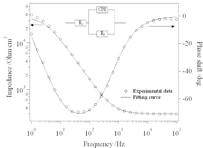
Fig. 11 Bode diagram of Al deposits obtained from the [EMIm]Cl/ AlCl_3 (0.5 mol%) bath using the MCP method with the conditions of r_C = 0.5 , f = 3.3 Hz.
