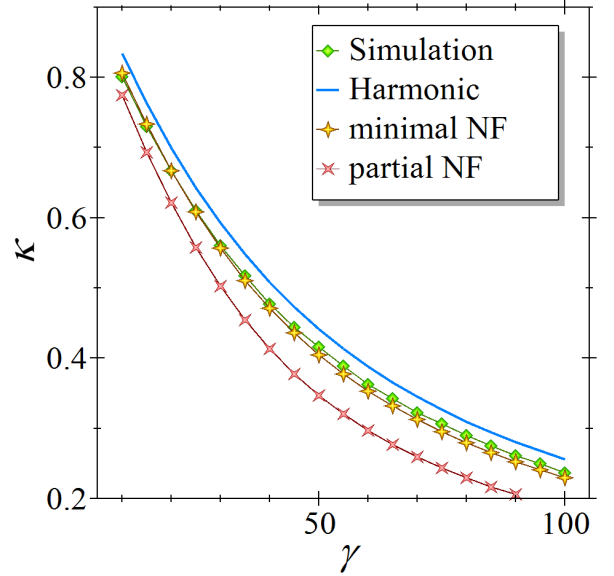
(b) k_B T = 5
