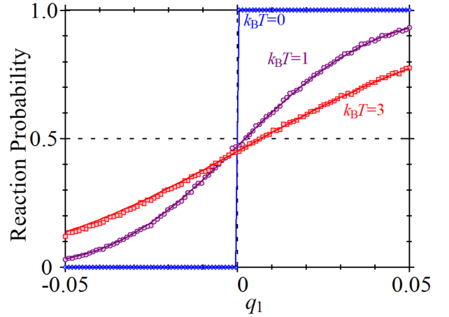
(b) Saddle 1, (q_2, \dot{q}_1, \dot{q}_2)|_{t=0} = (0.1, 0, 0)
