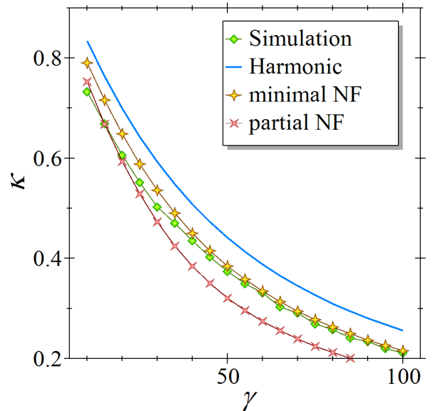
FIG. 2: Transmission coefficients calculated for saddle 2 of the Müller-Brown potential as functions of the friction constant \gamma . (a) k_B T = 3 , (b) k_B T = 5 . Green diamond: results of numerical simulations. Blue solid line: calculation by harmonic approximation. Yellow plus: minimal NF up to the second order perturbation. Red cross: partial NF up to the second order perturbation. harmonic approximation. Note that the partial NF shows poor performance, which is due to the worse convergence property compared with the minimal NF. At the higher temperature ( k_B T = 5 ), the results of minimal NF exhibit some deviations from the simulation, probably due to the insufficient order of the perturbation calculation performed. This shows that the condensed phase reaction probability based on the minimal NF proposed in this paper is appropriate to evaluate the effect
