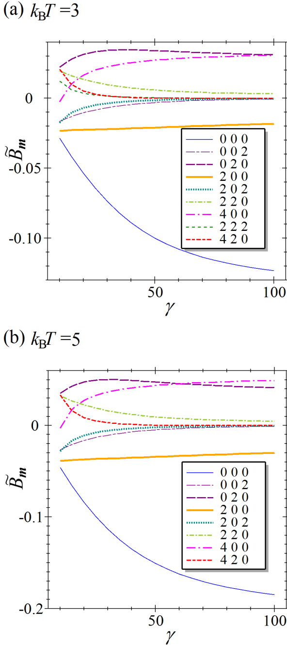
FIG. 3: Values of the coefficients appearing in the polynomial expression of the numerator of the transmission coefficients. (a) k_B T = 3 . All the other coefficients not shown are less than 0.012 in magnitude. (b) k_B T = 5 . All the other coefficients not shown are less than 0.02 in magnitude. The inset shows the corresponding powers of q_2, \dot{q}_1, \dot{q}_2 for each line.
