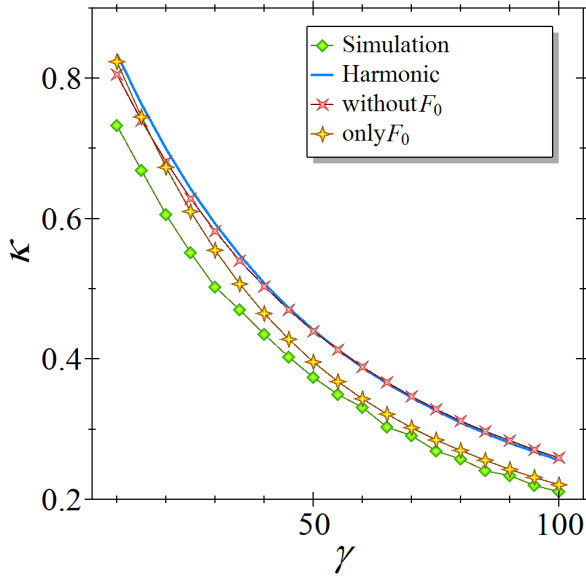
(b) k_B T = 5
