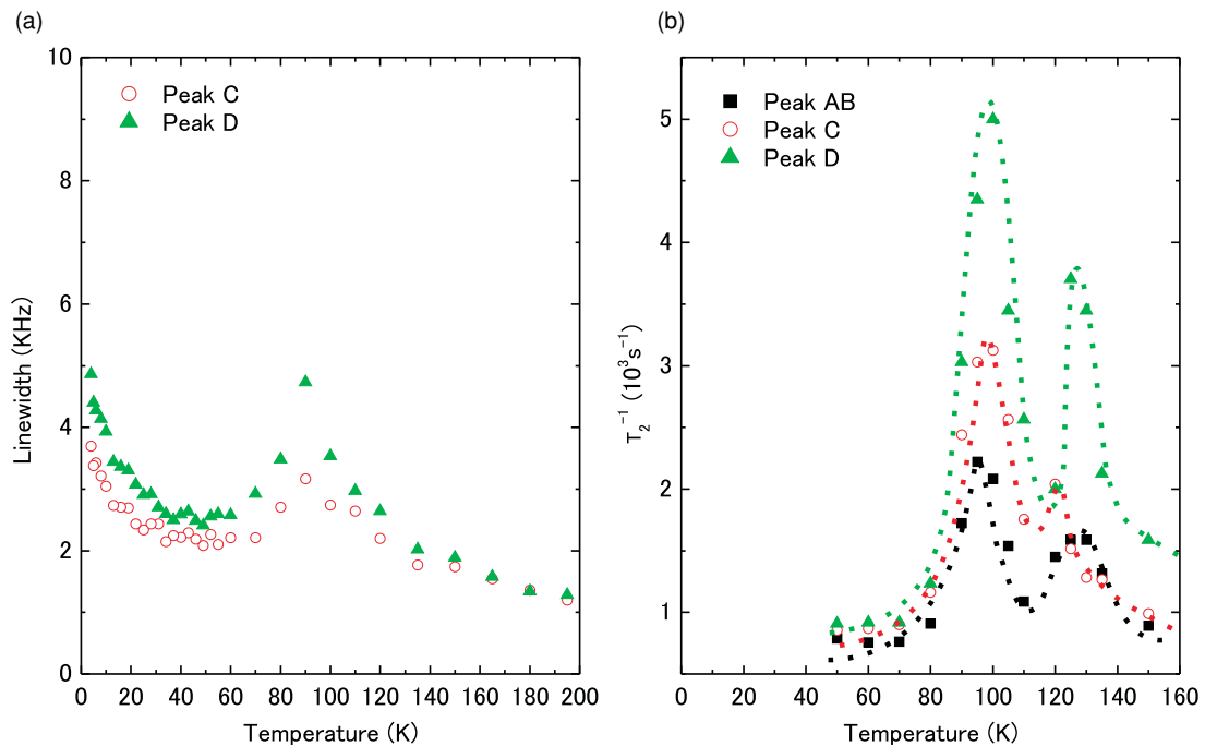
FIG. 2. (Color online) (a) Temperature dependence of the linewidths of the C and D sites in \kappa -(BEDT-TTF) _2\text{Cu}(\text{NCS})_2 . We could not evaluate the linewidths of the A and B sites because of their merged of peaks in the ^{13}\text{C} -NMR spectrum [Fig. 1(c)]. (b) Temperature dependence of T_2^{-1} in \kappa -(BEDT-TTF) _2\text{Cu}(\text{NCS})_2 . The dashed lines are guides to the eyes.
