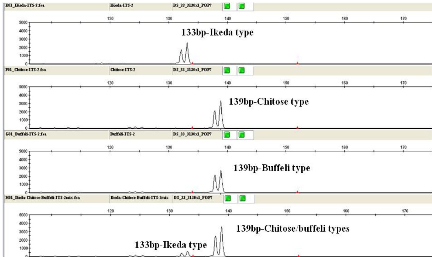
Fig 5: the three Theileria orientalis types on capillary electrophoresis genotyping plot by ITS2
