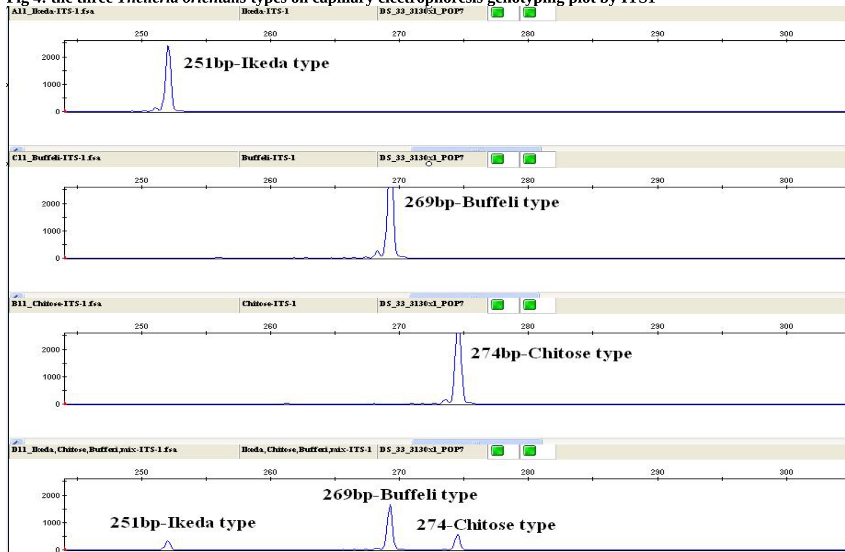
Fig 4: the three Theileria orientalis types on capillary electrophoresis genotyping plot by ITS1
