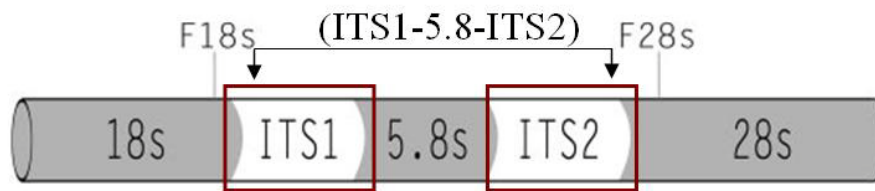
Fig 2: rRNA Internal transcribed spacer region and the Primer design target regions
