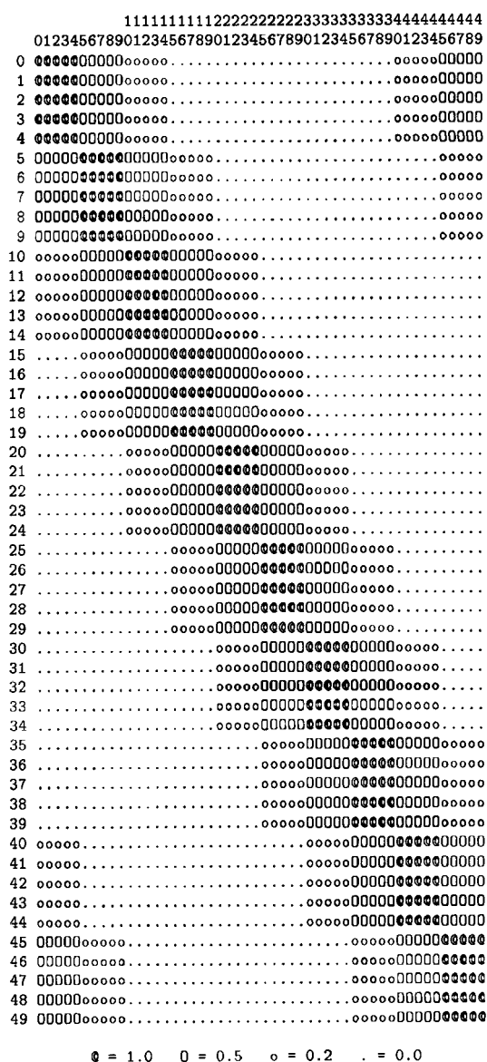
Figure 6: Tightness between loci for the 5-bit overlapping function ( \omega = 2.0 ).
