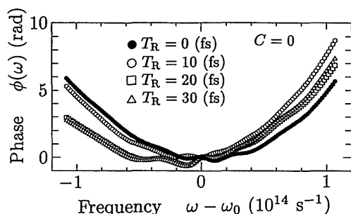
Fig. 2. Fiber output phase \phi(\omega) in the frequency domain at the optimum propagation lengths z_{\text{opt}} . The parameters are P_0 = 100 W, T_{p,\text{in}} = 100 fs, and C = 0 .
