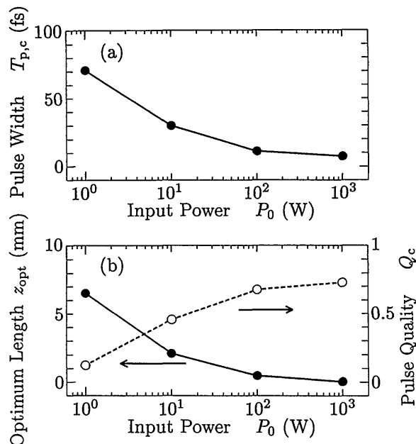
Fig. 3. Dependence of (a) the compressed pulse width T_{p,c} and (b) the optimum propagation length z_{\text{opt}} (filled circles) and the pulse quality Q_c (open circles) on the input power P_0 . The parameters are T_{p,\text{in}} = 100 fs, T_R = 0 fs, and C = 0 .
