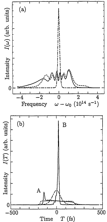
Fig. 1. (a) Typical fiber output spectra for response time T_R = 30 fs (solid curve) and T_R = 0 fs (dashed curve) at the distance z = 0.421 mm. The dotted-dashed curve represents the spectrum for the input pulse (input power P_0 = 100 W, pulse width T_{p,in} = 100 fs, and chirp parameter C = 0 ). (b) Typical fiber output pulses for T_R = 30 fs (solid curves: A, the precompensated pulse; B, the compensated pulse) and T_R = 0 fs (dashed curve, the precompensated pulse) at z = 0.421 mm. The dotted-dashed curve represents the input pulse. T is the time in the coordinate system moving at the average group velocity of the pulse.
