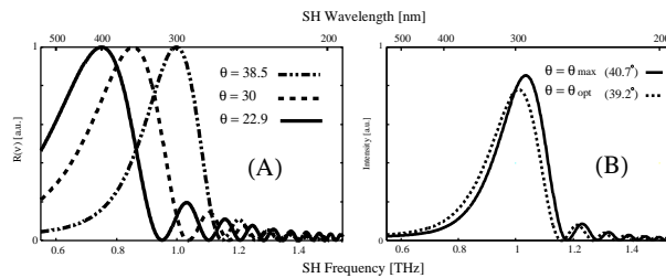
Fig. 4. Plots of the SH frequency-dependent filter function R(\Omega) of (A) normalized ones and (B) nonnormalized ones at various values of crystal angle \theta .
