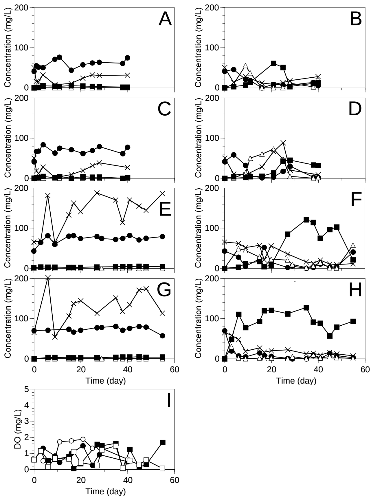
Fig.2 Macroscale and microscale analyses of nitrification and denitrification in biofilms attached on membrane aerated biofilm reactors. Hisashi Satoh et al.
