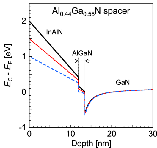
FIG. 5. (Color online) E_C potential profiles of the \text{In}_{0.18}\text{Al}_{0.82}\text{N} (12 nm)/ \text{Al}_{0.44}\text{Ga}_{0.56}\text{N} (1.5 nm)/GaN structure calculated for several E_F surf positions.
