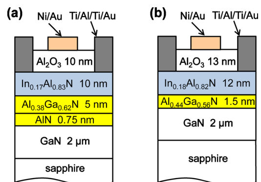
FIG. 1. (Color online) Schematic sample structures.
