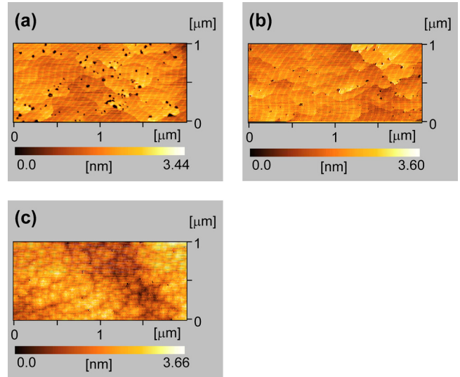
FIG. 4. (Color online) AFM images for (a) \text{Al}_{0.44}\text{Ga}_{0.56}\text{N} (2.0 nm)/ \text{GaN} , (b) \text{Al}_{0.44}\text{Ga}_{0.56}\text{N} (1.5 nm)/ \text{GaN} , and (c) \text{In}_{0.18}\text{Al}_{0.82}\text{N} (12 nm)/ \text{Al}_{0.44}\text{Ga}_{0.56}\text{N} (1.5 nm)/ \text{GaN} .
