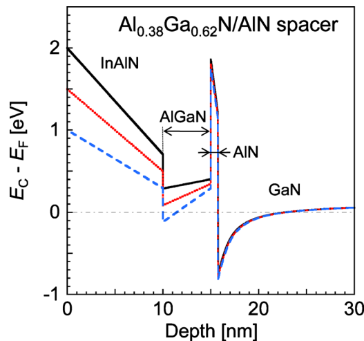
FIG. 3. (Color online) E_C potential profiles of the \text{In}_{0.17}\text{Al}_{0.83}\text{N} (10 nm)/ \text{Al}_{0.38}\text{Ga}_{0.62}\text{N} (5 nm)/ \text{AlN} (0.75 nm)/ \text{GaN} structure calculated for several E_{F\text{ surf}} positions.
