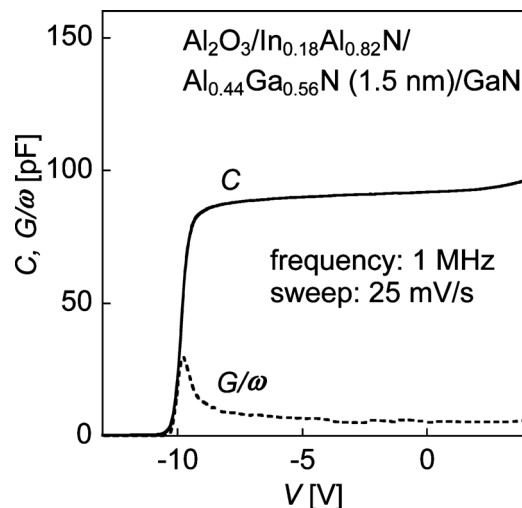
FIG. 6. Measured C-V curve for the \text{Al}_2\text{O}_3 (13 nm)/ \text{In}_{0.18}\text{Al}_{0.82}\text{N} (12 nm)/ \text{Al}_{0.44}\text{Ga}_{0.56}\text{N} (1.5 nm)/GaN structure. C_i was estimated to be \sim 190 pF. The bias voltage was swept from the positive side to the negative side at a sweep rate of 25 mV/s.
