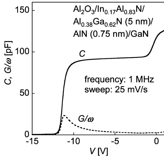
FIG. 2. Measured C-V curve for the \text{Al}_2\text{O}_3 (10 nm)/ \text{In}_{0.17}\text{Al}_{0.83}\text{N} (10 nm)/ \text{Al}_{0.38}\text{Ga}_{0.62}\text{N} (5 nm)/ \text{AlN} (0.75 nm)/ \text{GaN} structure. C_i was estimated to be \sim 260 pF. The bias voltage was swept from the positive side to the negative side at a sweep rate of 25 mV/s.
