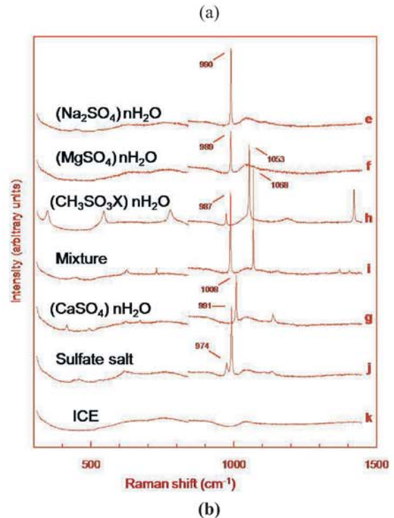
Fig. 3. Raman spectra of microparticles included in the Dome Fuji ice core [5]. The spectra e to i in panel (b) correspond to the optical microscope images (e) to (i) in panel (a), respectively. The hydration number n , unknown species X and unknown sulfate salt j are to be presented and discussed by Sakurai [15].
