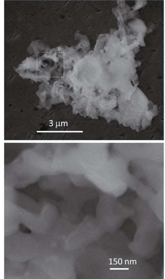
Fig. 7. FE-SEM images of a microparticle obtained by the sublimation method.
