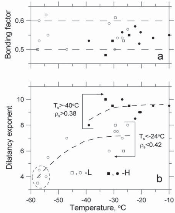
Figure 6: Critical bonding factor \zeta_0 (a) and dilatancy exponent \beta (b) for L-group (open symbols) and H-group (solid symbols) plotted against surface temperature. Squares and circles correspond to microstructural parameters constrained by direct stereological measurements and inferred from the density-depth profiles, respectively. Dashed lines show the range of \zeta_0 deviations in (a) and tendencies of \beta growth in (b).
