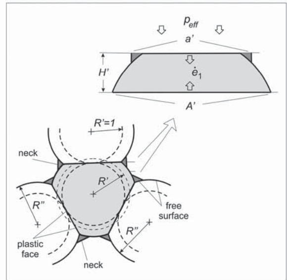
Figure 2: Modification of Arzt's geometric scheme [10] of ice-grain compaction by dislocation creep coupled with neck formation around plastic faces due to diffusive water-vapor transport. Inset: Deformation of a single spherical contact domain on a reference grain.
