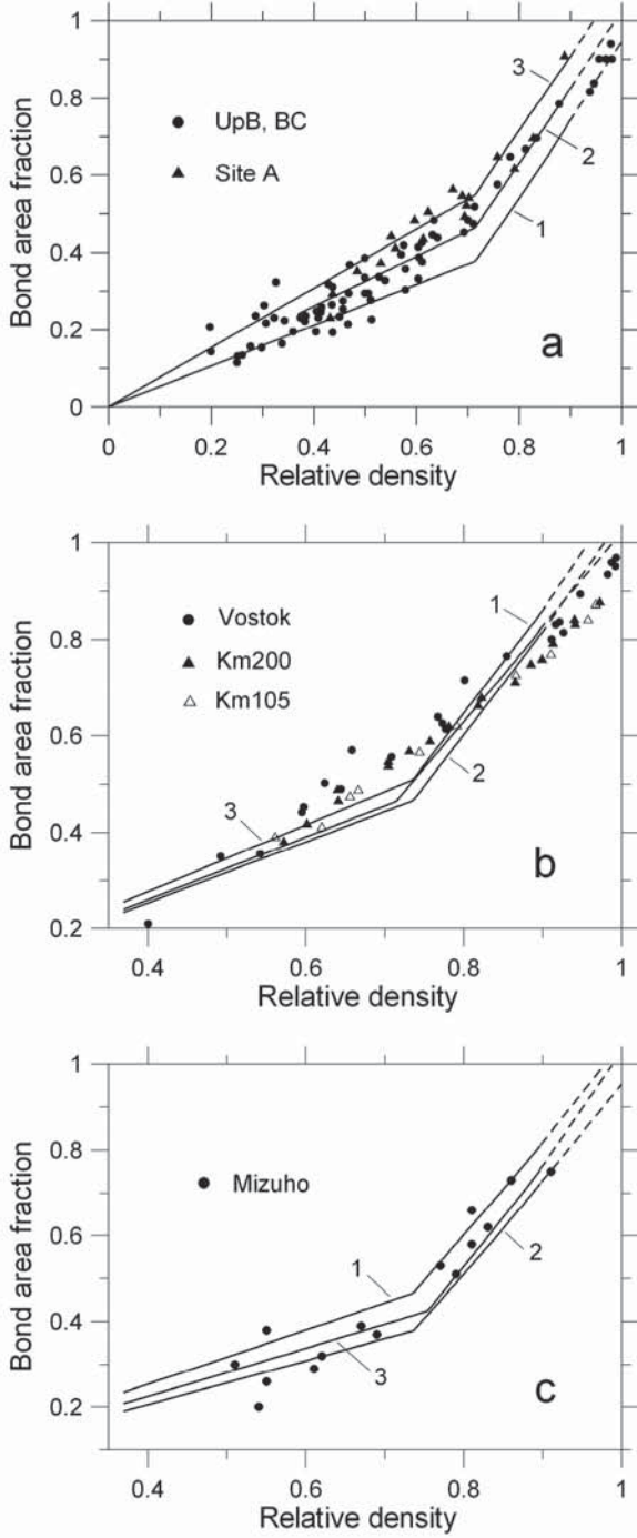
Figure 4: Bond area fraction versus relative density (symbols) for ice cores from (a) UpB, BC, and Site A [4, 5], (b) Vostok, KM200, and KM105 [7, 9], and (c) Mizuho [54] compared to model predictions (solid lines) for various ice core structures specified by different critical bonding factors: (a) Z_0 = 7 , C = 40 , (1) \zeta_0 = 0.4 , (2) \zeta_0 = 0.5 , (3) \zeta_0 = 0.6 ; (b) (1) Z_0 = 7 , C = 40 , \zeta_0 = 0.5 , (2) Z_0 = 7.5 , C = 50 , \zeta_0 = 0.5 , (3) Z_0 = 7.5 , C = 50 , \zeta_0 = 0.55 ; (c) (1) Z_0 = 7.5 , C = 50 , \zeta_0 = 0.5 , (2) Z_0 = 7.5 , C = 50 , \zeta_0 = 0.4 , (3) Z_0 = 8 , C = 60 , \zeta_0 = 0.45 .
