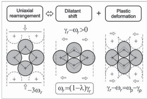
Figure 1: Interaction between dilatancy effects and plastic deviatoric deformations in snow densification by grain rearrangement. Only excess deviatoric creep compensating for lateral dilatant expansion is depicted in the last fragment.
