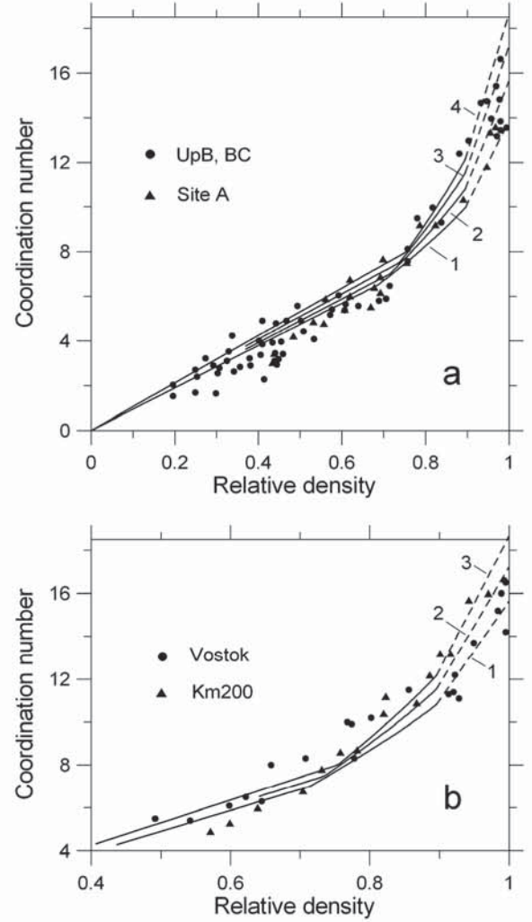
Figure 3: Coordination number versus relative density (symbols) for ice cores from (a) UpB, BC, and Site A [4, 5] and (b) Vostok and KM200 [7] compared to model approximations (solid lines) for various ice-core structures specified by critical microstructural parameters: (a) (1) Z_0 = 6.5 , C = 30 , (2) Z_0 = 7 , C = 40 , (3) Z_0 = 7.5 , C = 50 , (4) Z_0 = 8 , C = 60 ; (b) (1) Z_0 = 7 , C = 40 , (2) Z_0 = 7.5 , C = 50 , (3) Z_0 = 8 , C = 60 .
