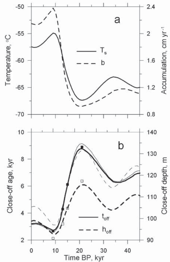
Figure 9: Paleoclimatic variations of close-off characteristics at Vostok Station for the last 45 kyr. (a) Ice-formation conditions ( T_s and b ) [72] and (b) quasi-stationary close-off depth h_{off} and ice age t_{off} calculated from Eqs. (25) (bold lines) and from the model [8] (thin lines), respectively. Open and solid squares denote h_{off} and t_{off} predicted by the proposed general model.
