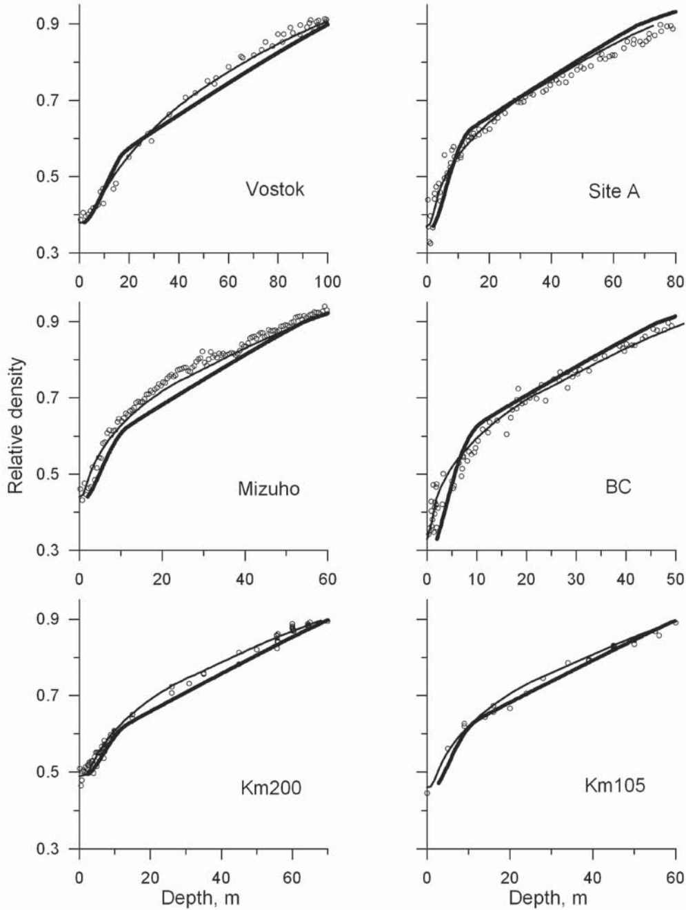
Figure 8: Comparison of density-depth profiles for basic ice cores from Vostok, Mizuho KM200, Site A, BC, and KM105 (thin solid lines) with the predictions of the model [8] (bold lines). Open circles denote experimental data (see Table 1).
