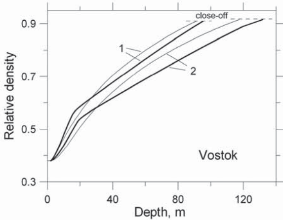
Figure 10: Quasi-stationary density-depth profiles at Vostok for the past temperature extremes at 9 and 21 kyr B.P. (curves 1 and 2, respectively) determined by the present model (thin lines) and by the model [8] (bold lines).
