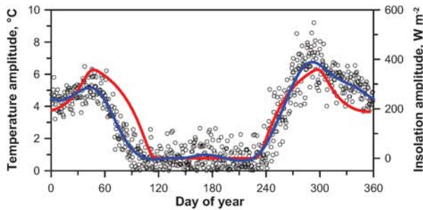
Figure 5: Diurnal amplitudes of measured air temperature [16] (black dots: daily averages over the period 1994 through 2001 based on 3 hourly air temperature data) and calculated local irradiation (red) assuming clear sky conditions at Dome Fuji. The blue line is the spline through the measurements.
