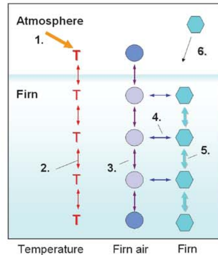
Figure 6: Schematic of total Temperature Gradient Metamorphism (tTGM) model: 1. Local insolation-air temperature; 2. Heat transfer; 3. Water vapour fluxes; 4. Water vapour pressure; 5. Density model; 6. Accumulation rates
