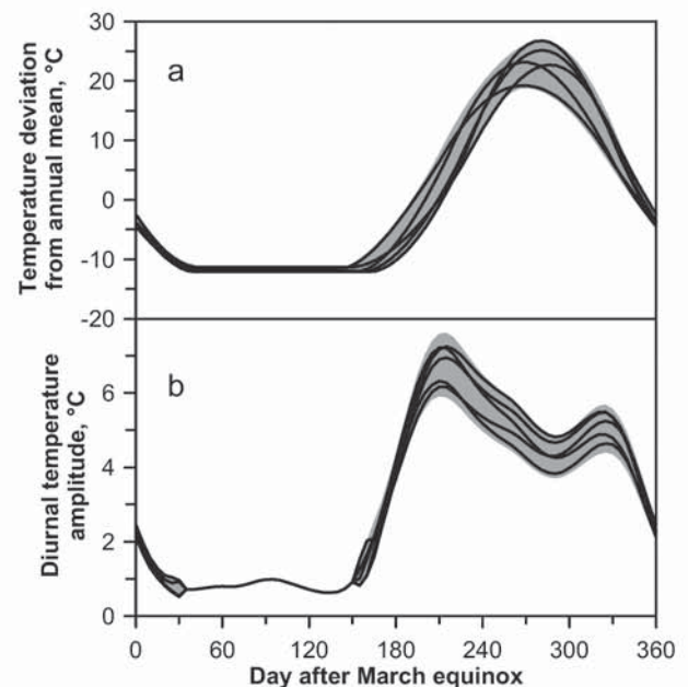
Figure 7: Range of calculated annual temperature cycles over the past 1 Ma at the snow surface (a). Corresponding range of the evolution of the
