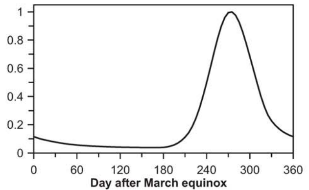
Figure 10: Normalized modelled total water vapour flux in the firn column in the course of the year for present day conditions. The sum of the total water vapour flux over the year corresponds by definition to tTGM (see text). Note that the higher values in autumn compared to spring are due to the summer
