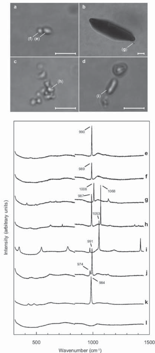
Figure 2: Micro-inclusions in the Dome Fuji ice core (left) and their Raman spectra (upper) [21]. (a) is ice from 362 m and the Holocene; (b), (c), and (d) are ice from 576 m, in the LGM. The large, black image in (b) is a plate-like inclusion; the rest of the others are micro-inclusions. The scale bar in each image is 10 \mu\text{m} . The Raman spectra of the labeled micro-inclusions are on the right. The spectra (e), (f), and (g) are assigned to \text{Na}_2\text{SO}_4 \cdot 10\text{H}_2\text{O} , \text{MgSO}_4 \cdot 12\text{H}_2\text{O} and \text{CaSO}_4 \cdot 2\text{H}_2\text{O} , respectively. (h) is assigned to a compound salt containing \text{SO}_4^{2-} and \text{NO}_3^- . (i) is assigned to a methanesulfonate salt. (j) is assigned to a sulfate salt. The cations and combined water of the salts (h)–(k) are not confirmed. (l) is a typical spectrum of the surrounding ice showing no significant peaks in this wavenumber range. Identification of the spectra (e)–(g) was based on data obtained from prepared reference samples. The classes of the salts (h)–(k) were inferred from their spectral features.
