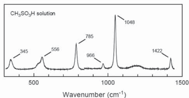
Figure 1a: Raman spectra of the reference specimen for \text{CH}_3\text{SO}_3\text{H} [21].
