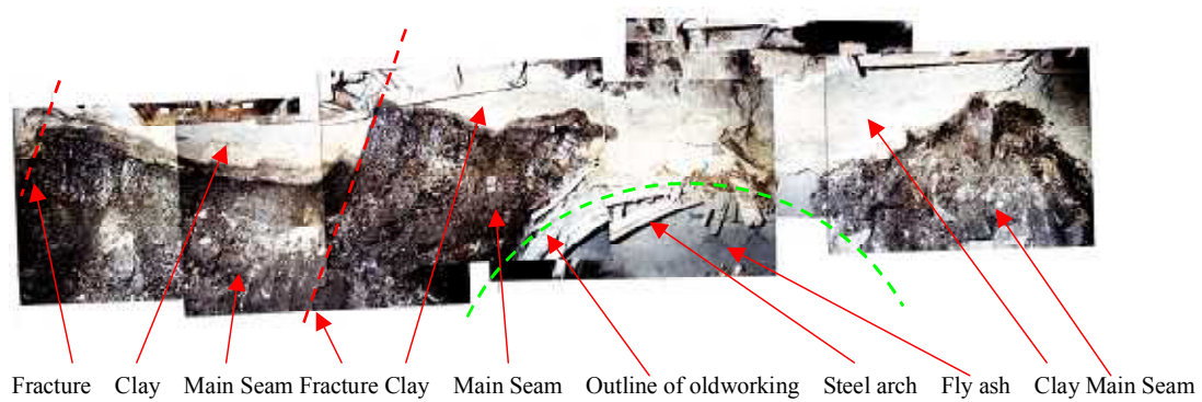
Fig. 13 Old roadway observed in Jobu Chuo No. 1 SD. Shear fractures and variation of clay thickness can be seen.
