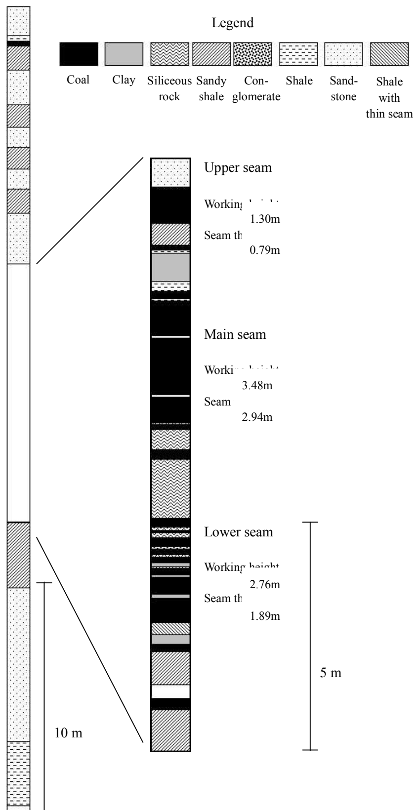
Fig. 1 Geological columnar section.
