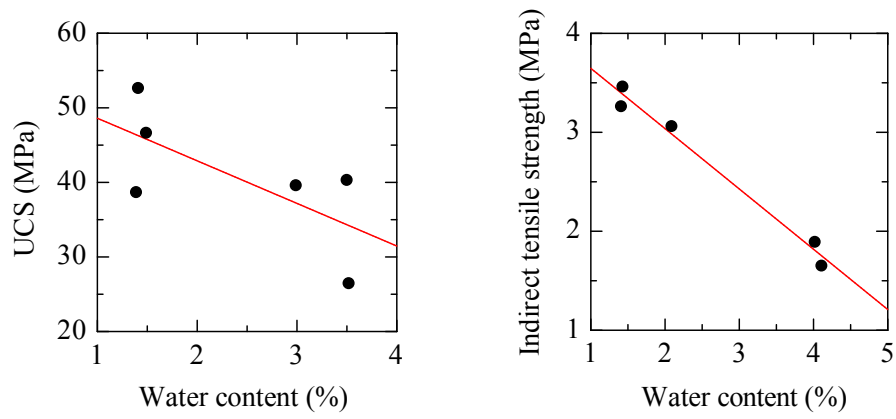
(a) Uniaxial compressive strength
