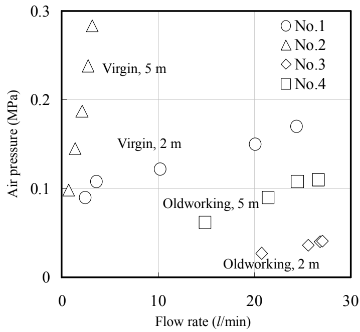
Fig. 16 Injection pressure vs. flow rate obtained by Lugeon test when the compressed air was used as fluid.
