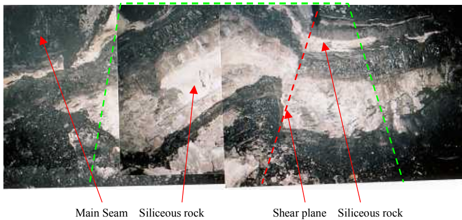
Fig. 6 Old roadway observed in Jobu Hidari No. 6 SD. The deflected floor was sheared. Variation in width of siliceous rock can be seen.
