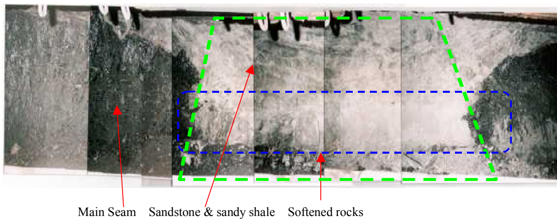
Fig. 7 Old roadway observed in Jobu Hidari No. 6 SD. Fragments of roof rock distributed in coal slurry (gray part seen around the top of the old roadway), the mixture of water and fine coal powder produced in coal processing.
