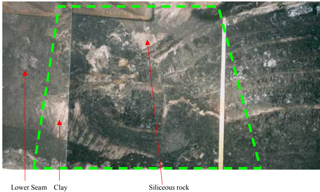
Fig. 5 Old roadway observed in Jobu Hidari Lower Seam No. 1 SD. Right part of the roof kept deflected shape. Left part was crushed by compression.
