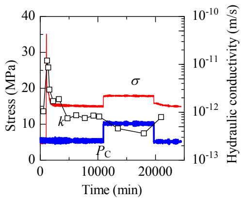
Fig. 19 Axial stress ( \sigma ), confining pressure ( P_c ) and hydraulic conductivity ( k ) versus time obtained under the triaxial compression test using sandstone.
