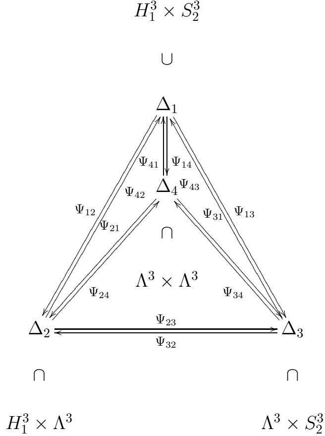
Fig. 1.1. The Mandala of Legendrian Dualities
