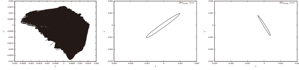
Figure 5: Chaotic attractor projected onto x - x^* plane and unstable periodic orbits near the attractor ( \mu = 0.022 ). Unstable periodic orbit with a positive correlation between x and x^* (middle: UPO_{3.0165} ); unstable periodic orbit with a negative correlation between x and x^* (right: UPO_{3.0148} ).
