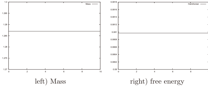
Figure 2. The computed value Mass and free energy for Problem
